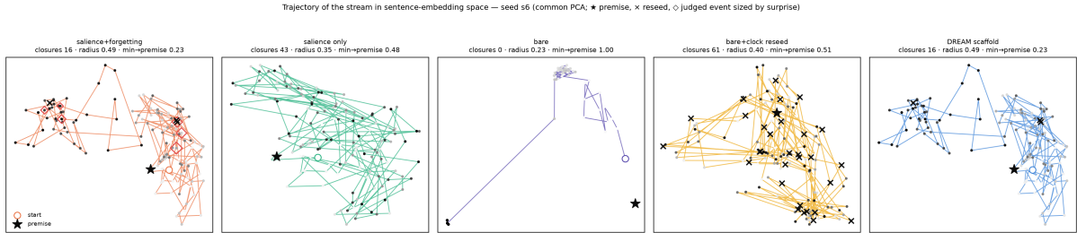
Figure 5: Where the stream goes: trajectories in sentence-embedding space (64-token windows, one PCA per seed), seed 6. \star premise, \circ start, \times reseed, \diamond judged event sized by surprise. Bare makes one jump and freezes; the scaffold orbits and returns; the clock reseed jumps across the space keeping its context.
