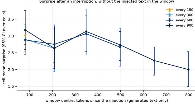
Figure 11: Decay: cell-mean surprise of generated-only windows by tokens since the injection, per period.
