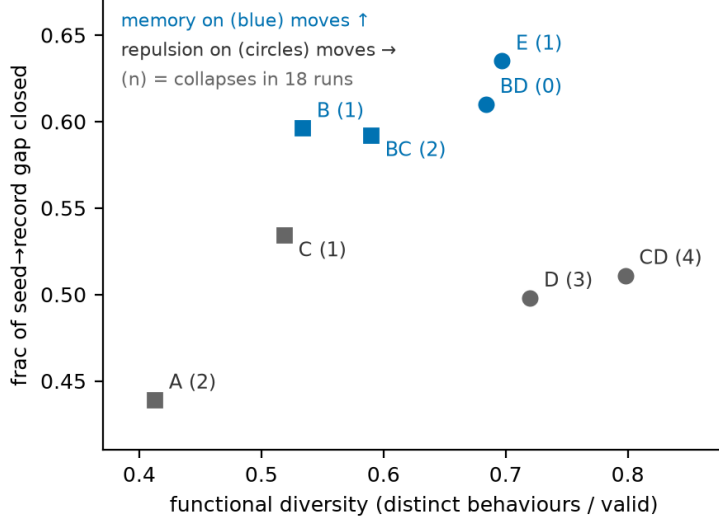
Figure 1: The completed 2^3 at a glance (cell means over nine problems, two replicates). Memory-on cells (blue) hold the four best gap fractions; repulsion-on cells (circles) hold the highest functional diversity; the two axes barely interact ( \beta_{M \times R} \approx 0 ). Collapse counts in parentheses: memory+repulsion is the only arm that never collapses; agenda+repulsion collapses most.
