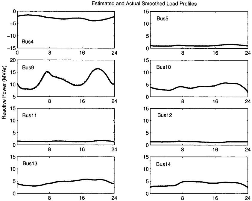
Figure 13.8. Comparisons between smoothed original and estimated reactive load profiles.
