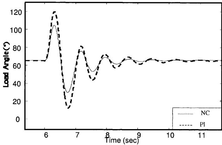
Figure 10.22. Load angle response of the synchronous generator operating ( P = 0.65 p.u. and Q = 0.12 p.u.) for a 180 ms three phase short circuit at Bus 2.
