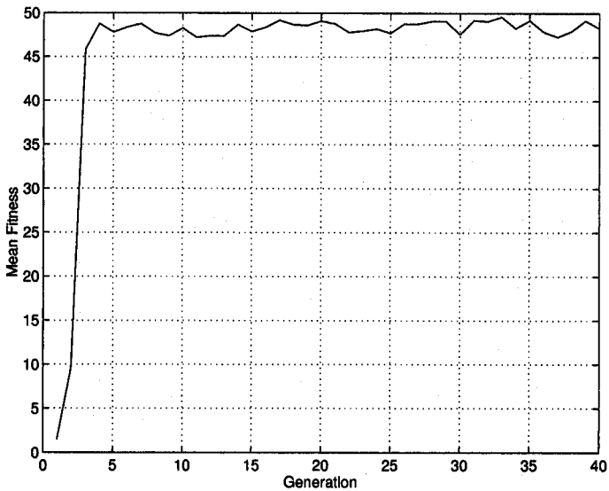
Figure 11.11. GA convergence performance.
