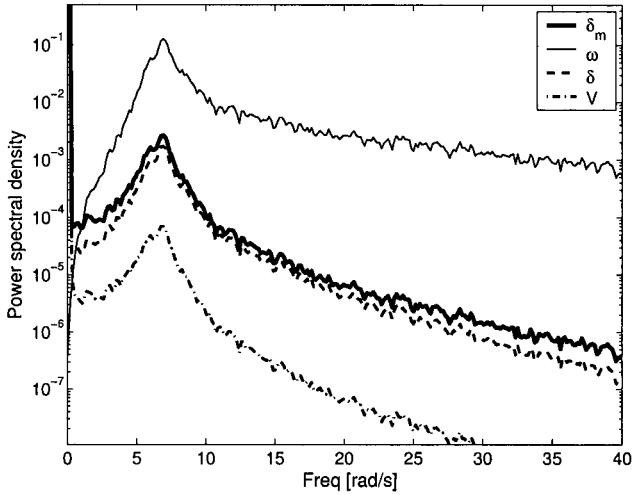
Figure 8.2. Power spectral densities of the states of the model given in (8.16)-(8.19). The bifurcation parameter was set to Q_1 = 2.9 . White Gaussian noise of zero mean and (0.001)^2 power was added to P_m .
