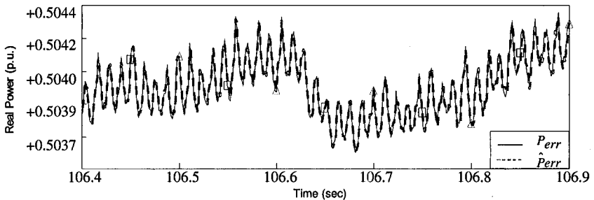
Figure 10.17. Actual signal P_{err}(t) of the plant and estimated signal \hat{P}_{err}(t) by the SENI.
