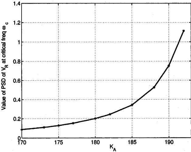
Figure 8.6. Variation of the peak value of the power spectral density of V_R as a function of the bifurcation parameter K_A . White Gaussian noise of zero mean and (0.000032)^2 power was added to P_m .
