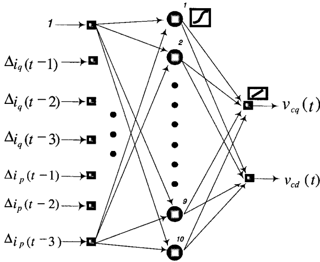
Figure 10.26. Input-output mapping of the action network at t used in the critic network adaptation in Figure 10.24. A(t) in Figure 10.24 is v_{cq}(t) and v_{cd}(t) .
