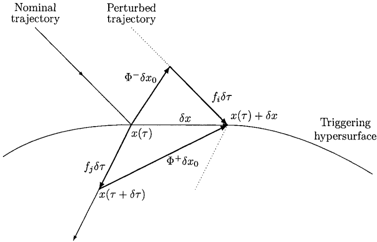
Figure 9.1. Jump conditions.
