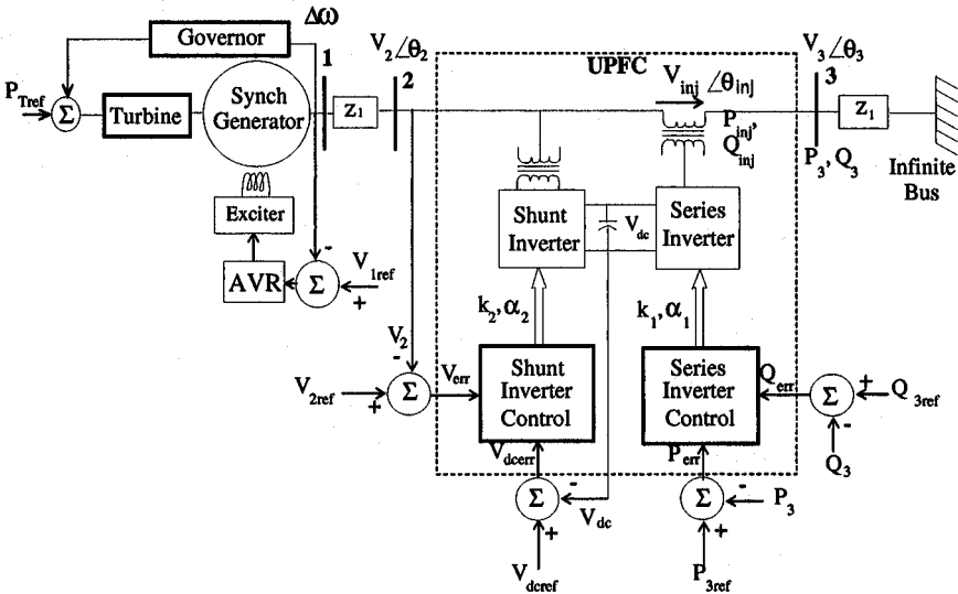
Figure 10.5. Single machine infinite bus power system with a UPFC (dashed lines show the “plant”).
