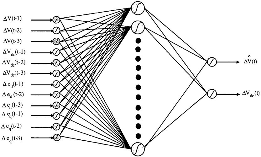
Figure 10.9. Neuroidentifier structure for a STATCOM neurocontroller design.
