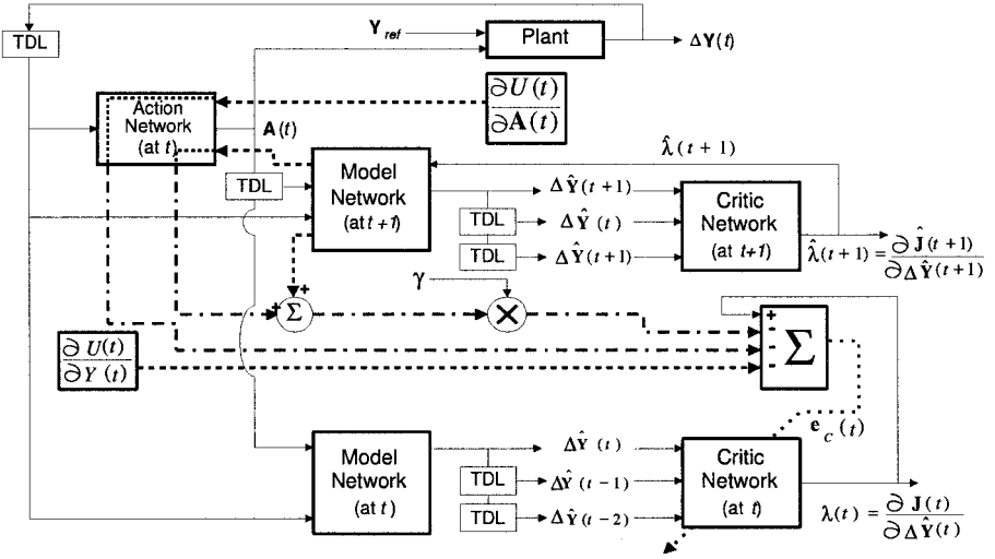
Figure 10.24. Critic network adaptation in DHP showing the implementation of (10.21).
