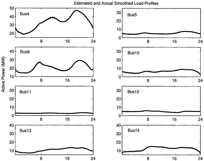
Figure 13.5. Comparison of smoothed original signals and estimated signals.
