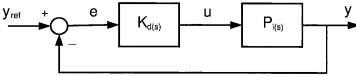
Figure 11.9. Closed-loop setup.
