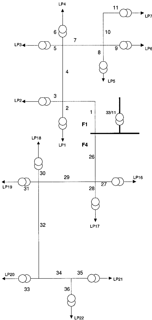
Figure 11.8. System used in Example 2.
