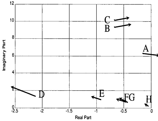
Figure 4.4. All complex eigenvalues in complex plane at base case.
