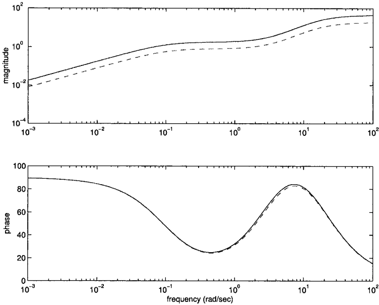
Figure 11.13. Frequency response of the nominal TCSC POD controller (dashed line) and the GA-designed TCSC POD controller (solid line).
