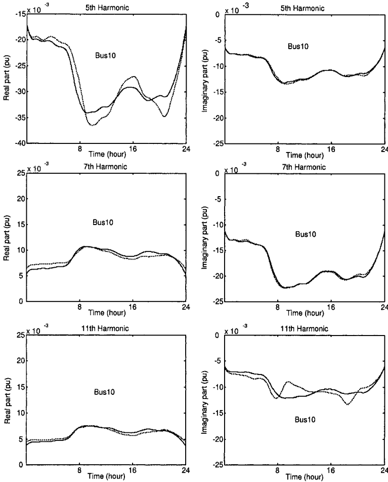
Figure 13.11. Comparison of smoothed harmonic components of current injection at Bus 10.
