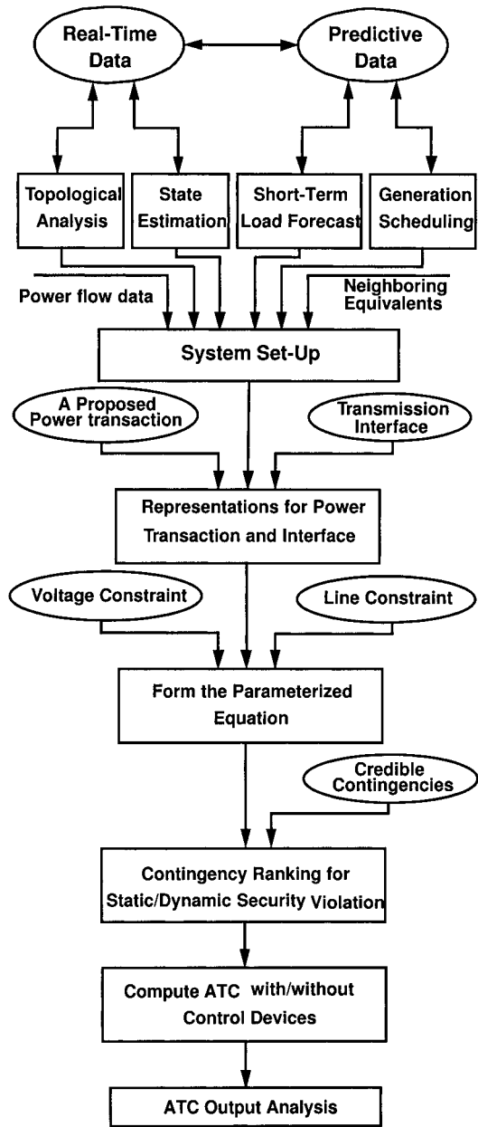
Figure 5.10. The overall architecture of the proposed tool for accurate evaluation of ATC.
