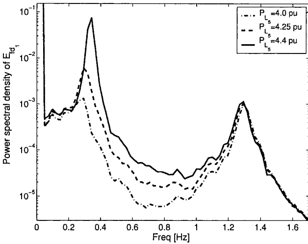
Figure 8.9. Power spectral density of E_{fd1} for three values of P_{L5} (the load on Bus 5): P_{L5} = 4.0 p.u. (dash-dotted line), P_{L5} = 4.25 p.u. (dashed line), and P_{L5} = 4.4 p.u. (solid line). White Gaussian noise of zero mean and 0.05 power was added to P_{m3} , the mechanical power of generator 3.
