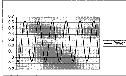
Figure 2.2. Instantaneous power.
