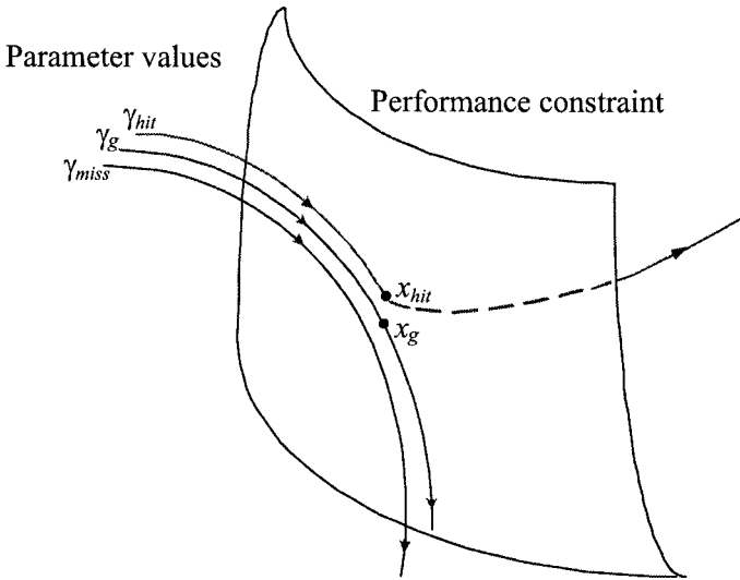
Figure 9.6. Grazing phenomenon.
