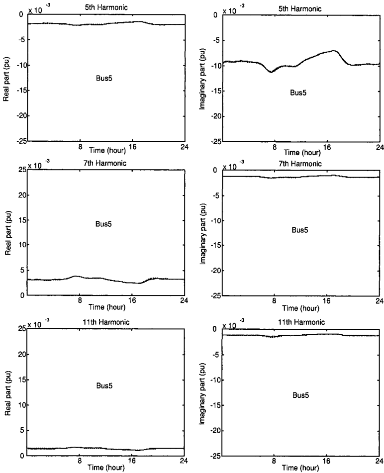
Figure 13.10. Comparison of smoothed harmonic components of current injection at Bus 5.
