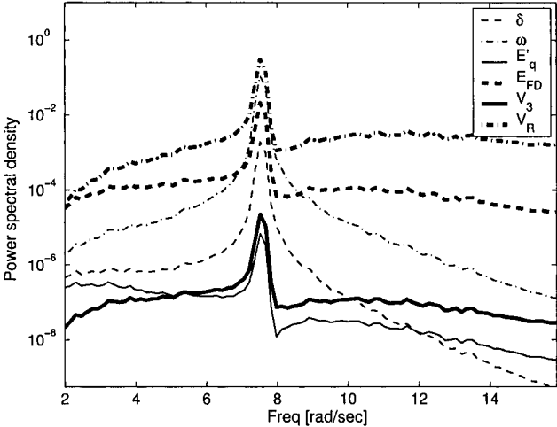
Figure 8.5. Power spectral densities of the states of the single generator connected to an infinite bus system. The bifurcation parameter was set to K_A = 185 . White Gaussian noise of zero mean and (0.000032)^2 power was added to V_{ref} .
