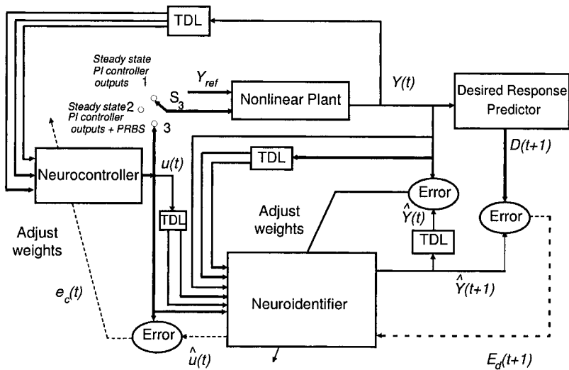
Figure 10.8. Indirect adaptive neurocontroller design structure for a nonlinear plant consisting of a neuroidentifier and a desired response predictor.
