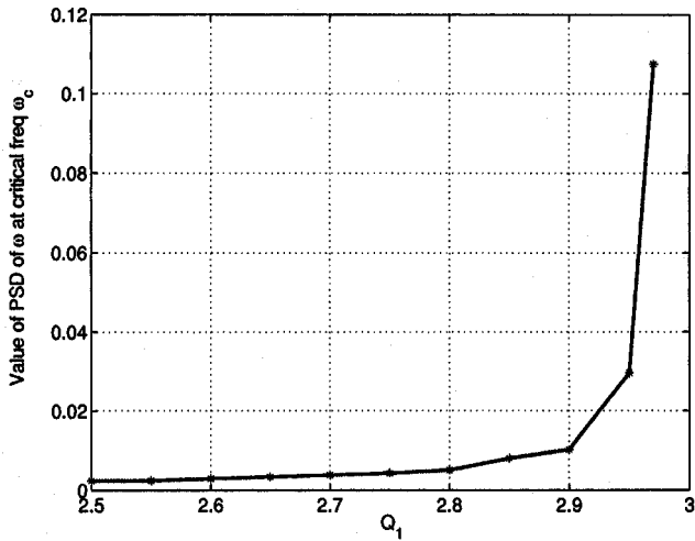
Figure 8.3. Variation of the peak value of the power spectral density of \omega as a function of the bifurcation parameter Q_1 . White Gaussian noise of zero mean and (0.001)^2 power was added to P_m .
