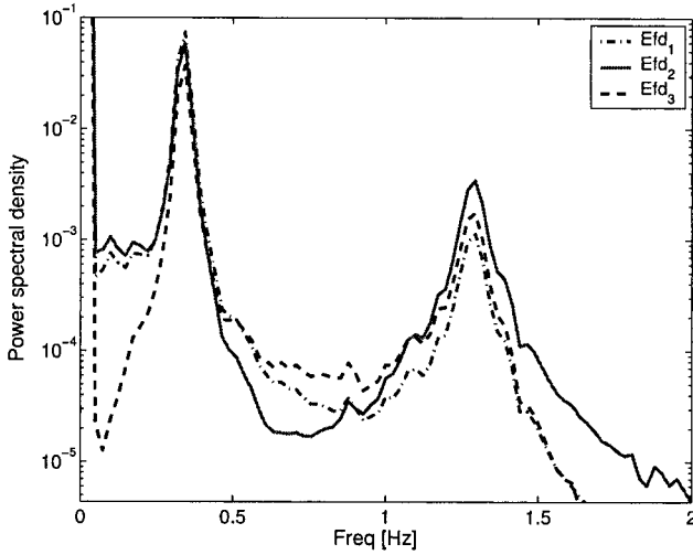
Figure 8.8. Power spectral densities of the states E_{fd1} , E_{fd2} , and E_{fd3} . The load on Bus 5 was used as a bifurcation parameter. The load value is 4.4 p.u. White Gaussian noise of zero mean and 0.05 power was added to P_{m3} , the mechanical power of generator 3.
