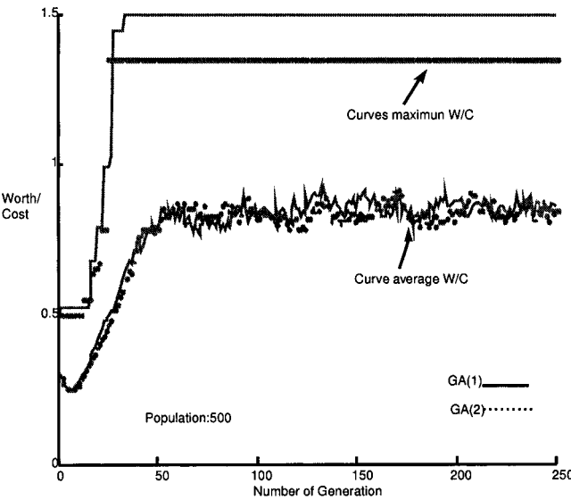
Figure 11.5. Maximum and average fitness in Example 1.
