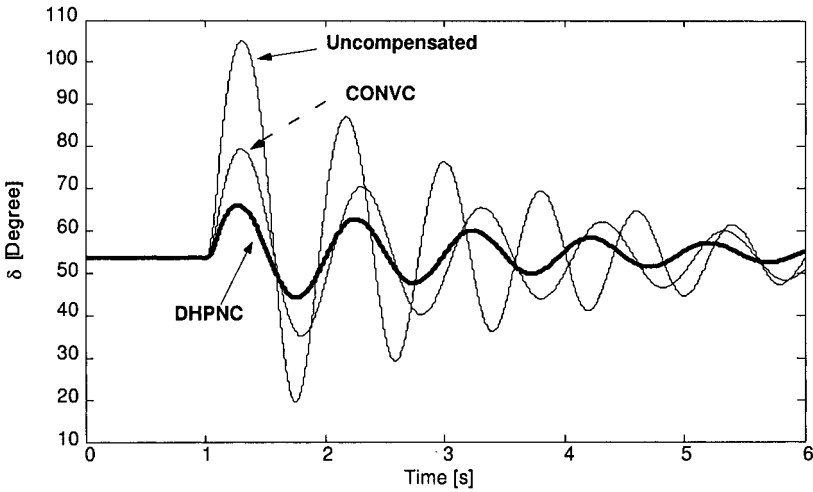
Figure 10.29. A 100 ms three phase short circuit test: \delta .
