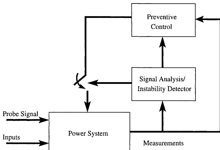
Figure 8.1. Precursor-based instability monitor with external probe signal.
