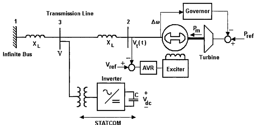
Figure 10.1. STATCOM connected to SMIB system (plant).
