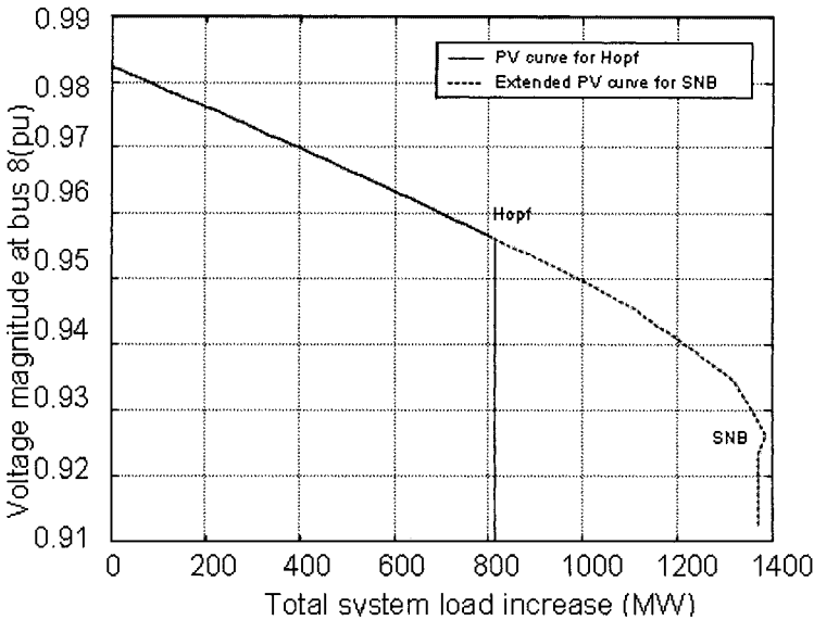
Figure 4.7. Hopf and SNB detection in PV curve tracing for base case control.
