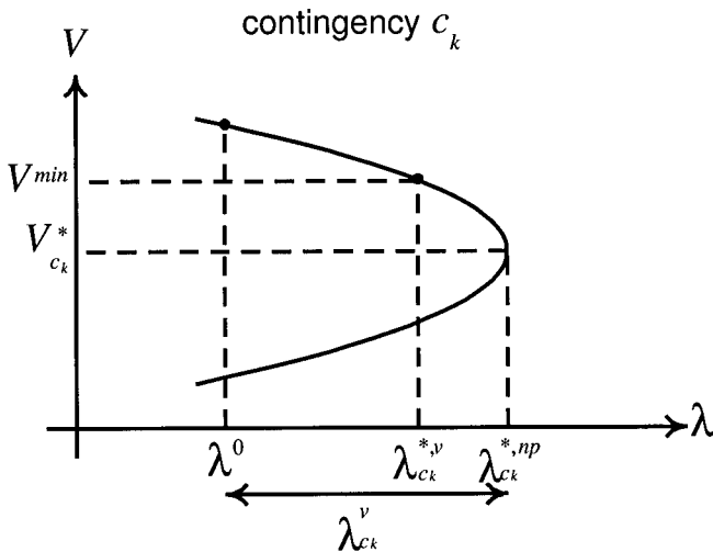
Figure 5.4. The voltage-limit load margin \lambda_{C_k}^v for the power system under contingency C_k .
