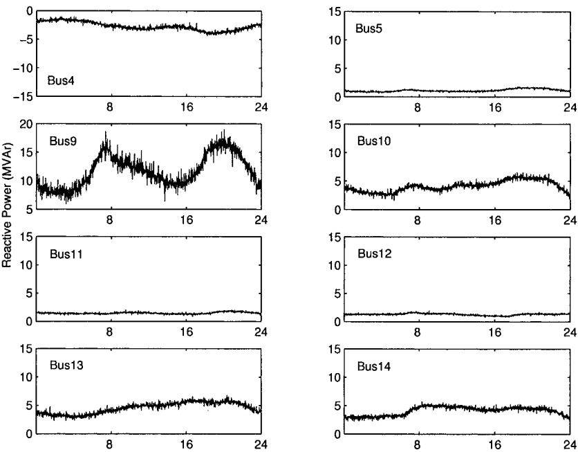
Figure 13.6. Original source signals: Reactive load profiles.
