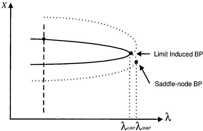
Figure 5.8. The limit-induced bifurcation point is close to the saddle-node bifurcation point.
