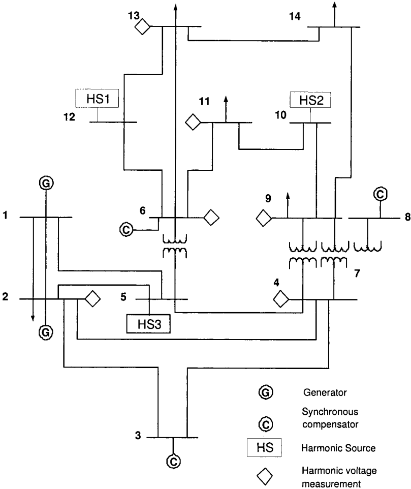
Figure 13.9. Modified IEEE 14-bus test system.
