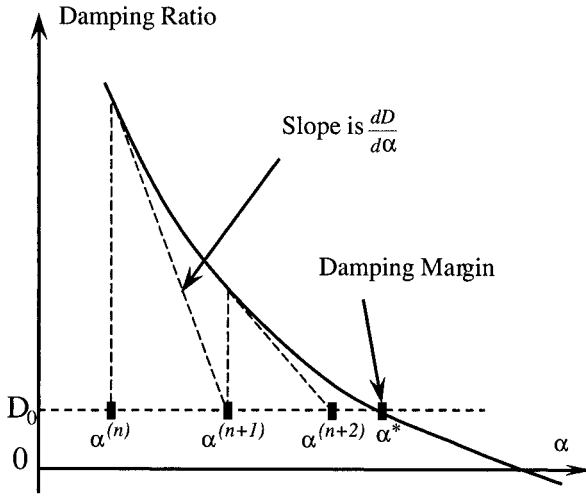
Figure 4.3. Tangent information is used in searching for damping margin.
