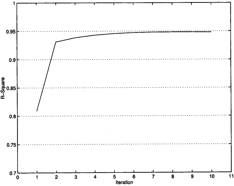
Figure 12.3. Convergence of the R^2 for the actual load vs the model.
