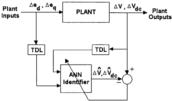
Figure 10.10. Neuroidentifier training for a STATCOM neurocontroller design.
