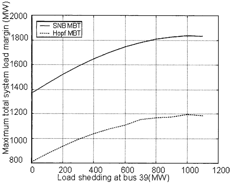
Figure 4.8. Margin boundary tracing (MBT) vs. load shedding.
