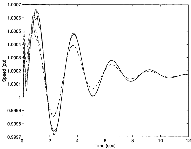
Figure 11.15. Rotor speeds for the load-switching simulation using the GA-designed SVC and TCSD POD controllers.
