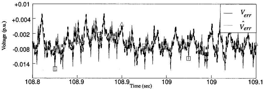
Figure 10.19. Actual signal V_{dcerr}(t) of the plant and estimated signal \hat{V}_{dcerr}(t) by the SHNI.
