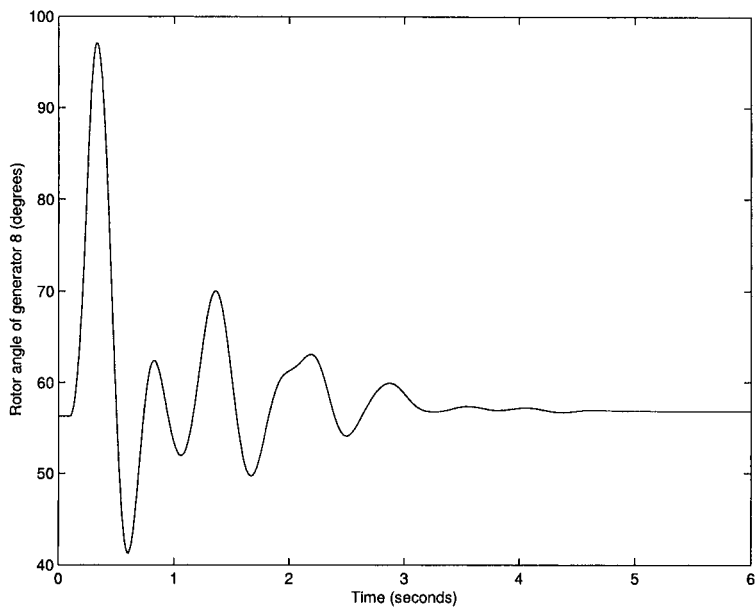
Figure 7.1. Rotor angle of Generator 8.
