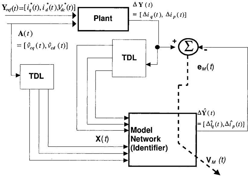
Figure 10.28. NARMAX model for on-line training of the model network.
