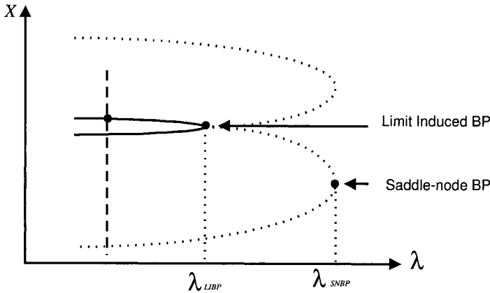
Figure 5.7. The limit-induced bifurcation point is far away from the saddle-node bifurcation point.
