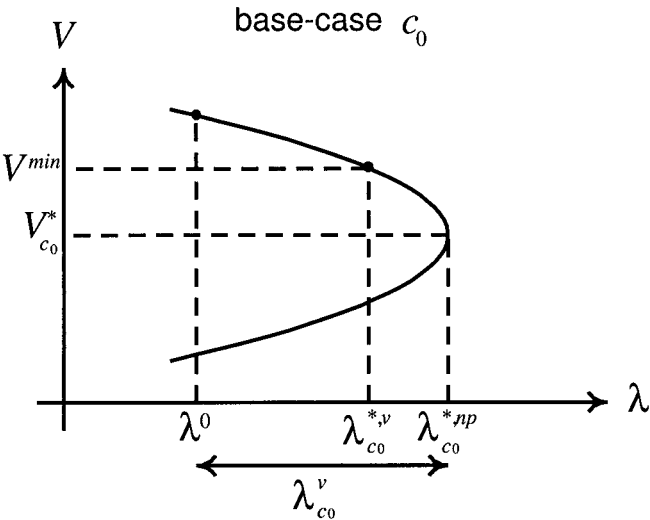
Figure 5.3. The voltage-limit load margin \lambda_{C_0}^v for the base case power system C_0 .
