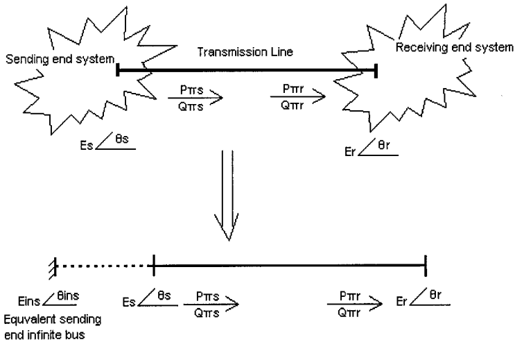
Figure 3.3. Simplify large scale power system to equivalent two-bus system.
