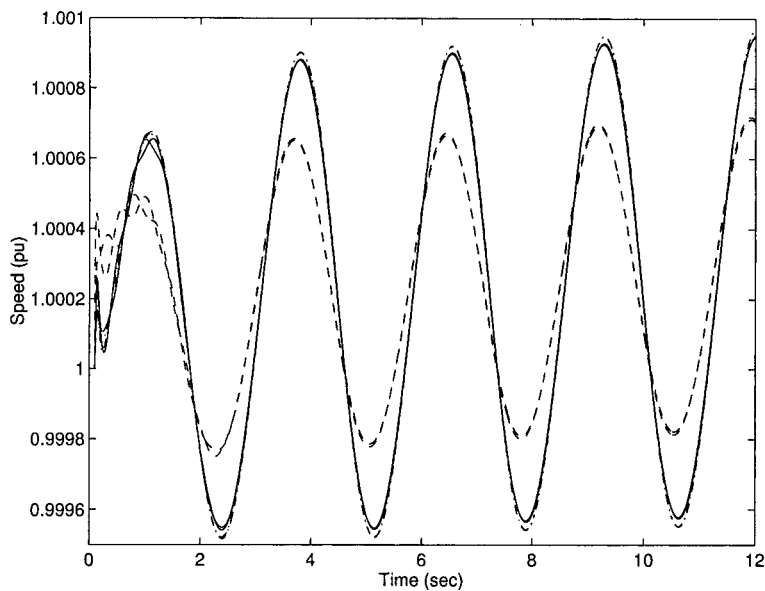
Figure 11.14. Rotor speeds for the load-switching simulation using the nominal SVC and TCSD POD controllers.
