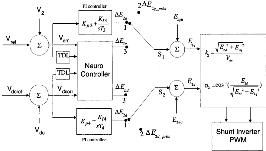
Figure 10.7. Shunt inverter control with conventional PI controllers and neurocontroller (TDL means tapped delayed lines).
