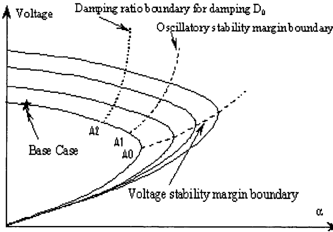
Figure 4.1. Illustration of three types of boundaries.
