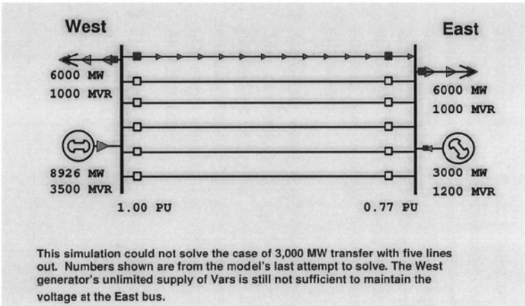
Figure 2.9. Illustration Case 6 (five lines out).
