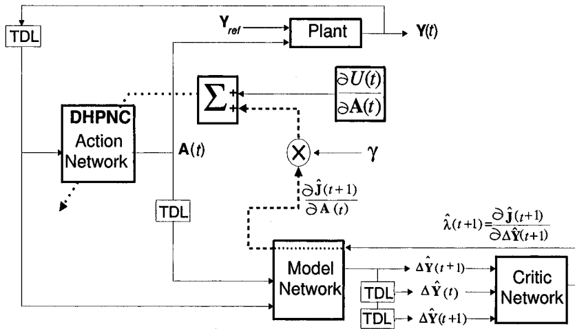
Figure 10.27. Action network adaptation in DHP.
