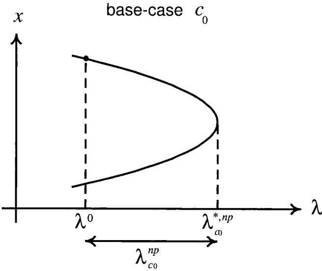
Figure 5.1. The nose point load margin \lambda_{C_0}^{np} for the base case power system C_0 .
