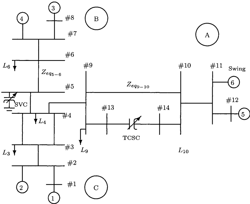
Figure 11.10. Three-area six-machine power system
