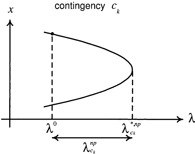
Figure 5.2. The nose point load margin \lambda_{C_k}^{np} for the power system under contingency C_k .
