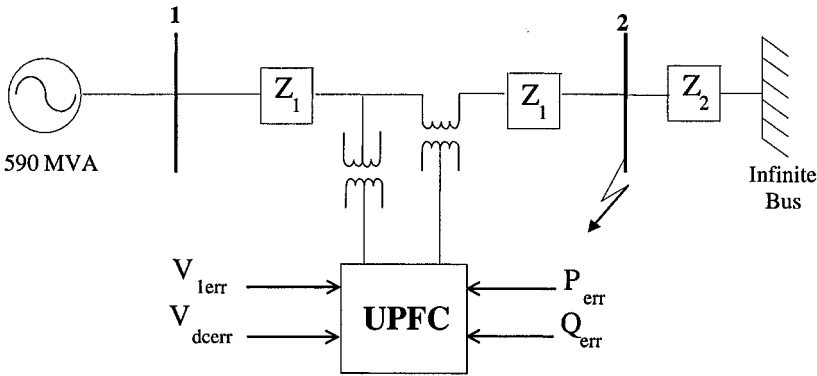
Figure 10.16. Single machine infinite bus power system with a single transmission line and a UPFC.
