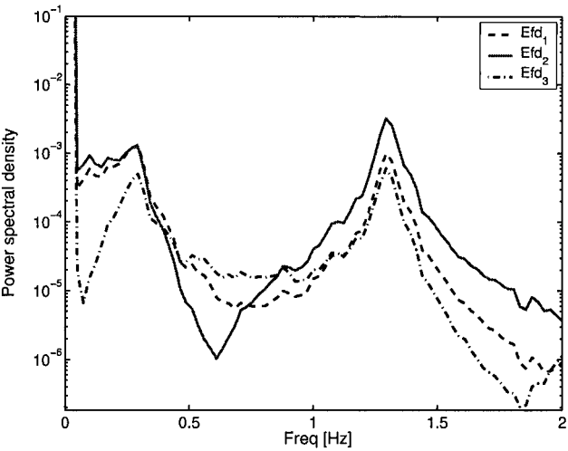
Figure 8.7. Power spectral densities of the states E_{fd_1} , E_{fd_2} , and E_{fd_3} . The load on Bus 5 was used as a bifurcation parameter. The load value is 4.0 p.u. White Gaussian noise of zero mean and 0.05 power was added to P_{m_3} , the mechanical power of generator 3.
