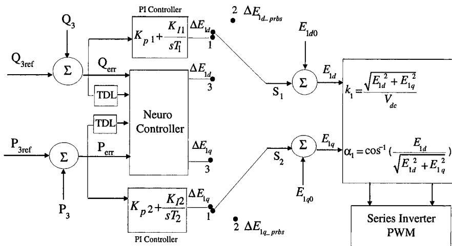
Figure 10.6. Series inverter control with conventional PI controllers, with neuro-controller and the inputs to the neurocontroller including two previous time delayed values of the signals (TDL means tapped delayed lines).
