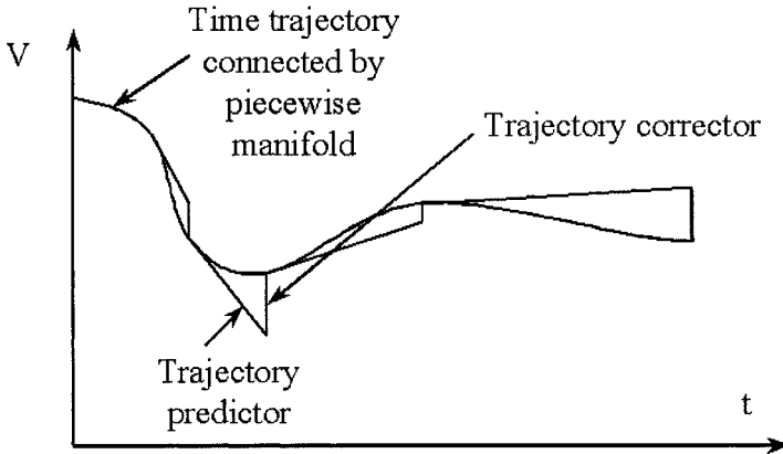
Figure 4.9. Continuation-based time domain simulation using locally parameterized time trajectory tracing.
