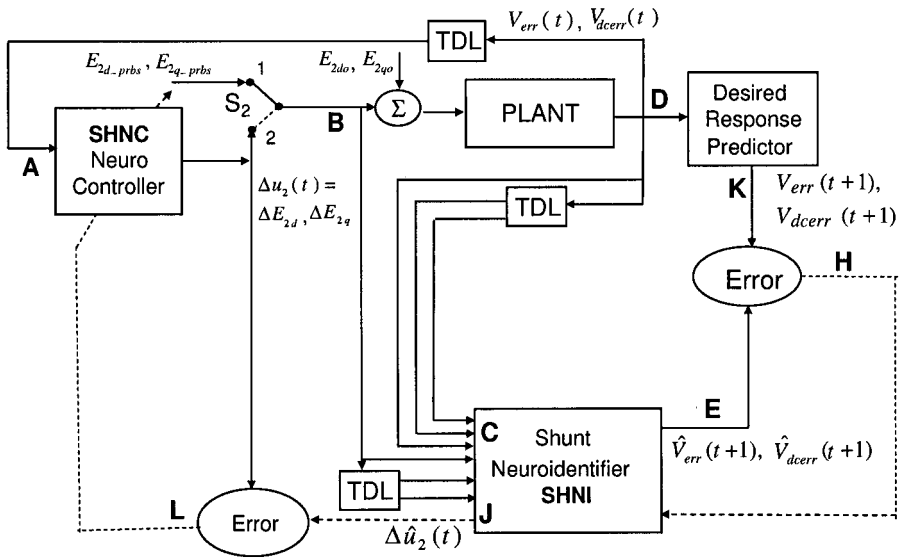
Figure 10.15. Training of SHNC to update its weights by backpropagating the error signals at L.
