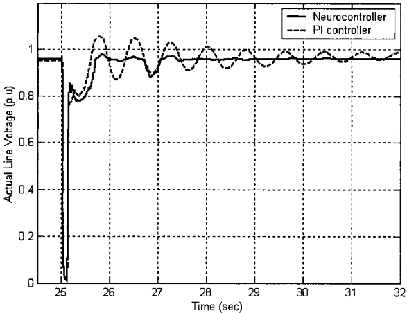
Figure 10.12. Line voltage during a 100 ms three-phase short circuit at the midline.
