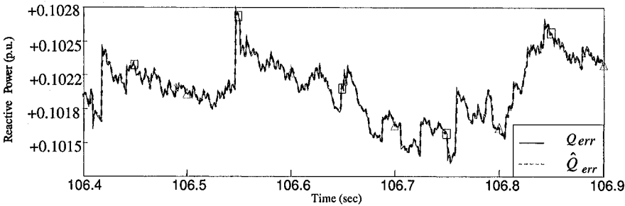
Figure 10.18. Actual signal Q_{err}(t) of the plant and estimated signal \hat{Q}_{err}(t) by the SENI.
