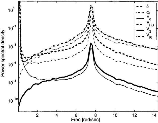
Figure 8.4. Power spectral densities of the states of the single generator connected to an infinite bus system. The bifurcation parameter was set to K_A = 185 . White Gaussian noise of zero mean and (0.000032)^2 power was added to P_m .
