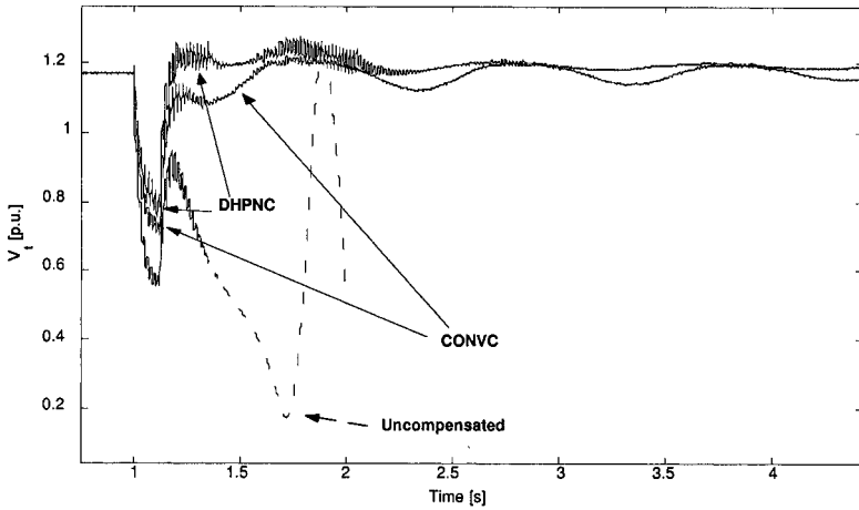
Figure 10.32. A 120 ms three phase short circuit test: V_t .
