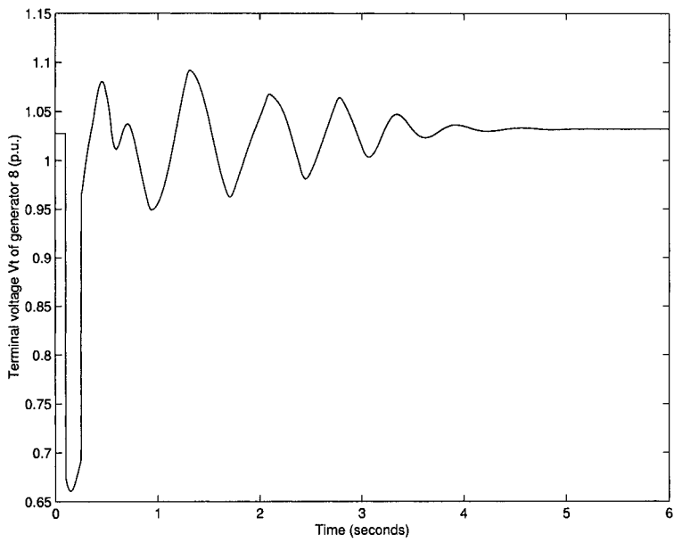
Figure 7.2. Terminal voltage V_t of Generator 8.
