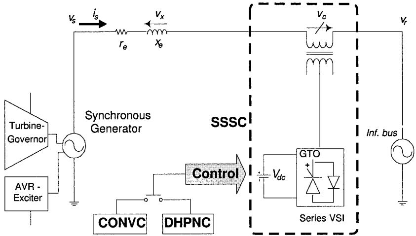
Figure 10.3. Plant: 160 MVA, 15 kV (L-L) SMIB test system.
