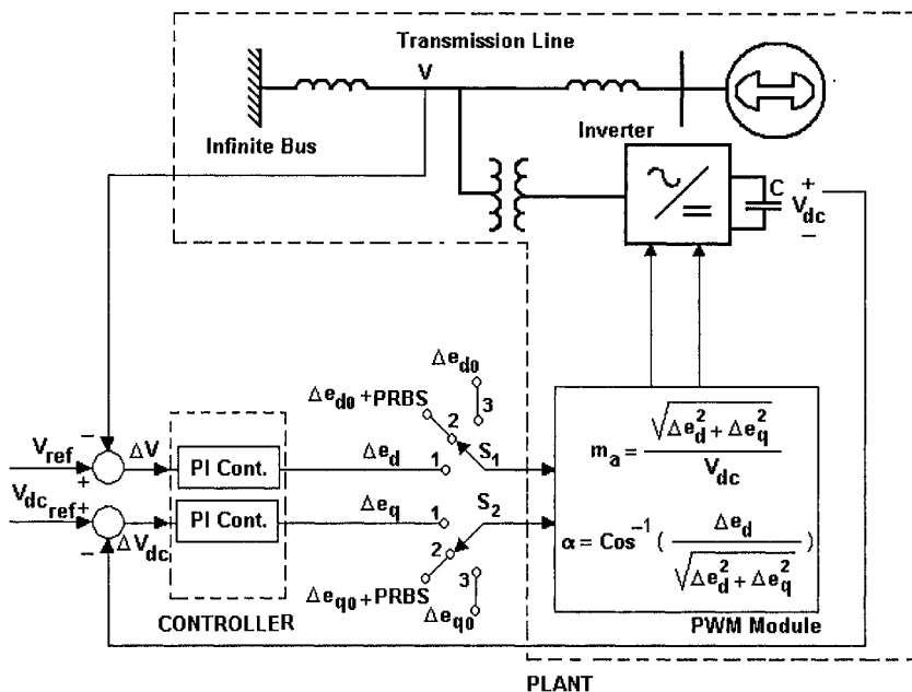
Figure 10.2. STATCOM controller.
