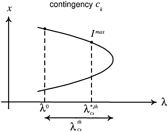
Figure 5.6. The thermal-limit load margin \lambda_{C_k}^{th} for the power system under contingency C_k .
