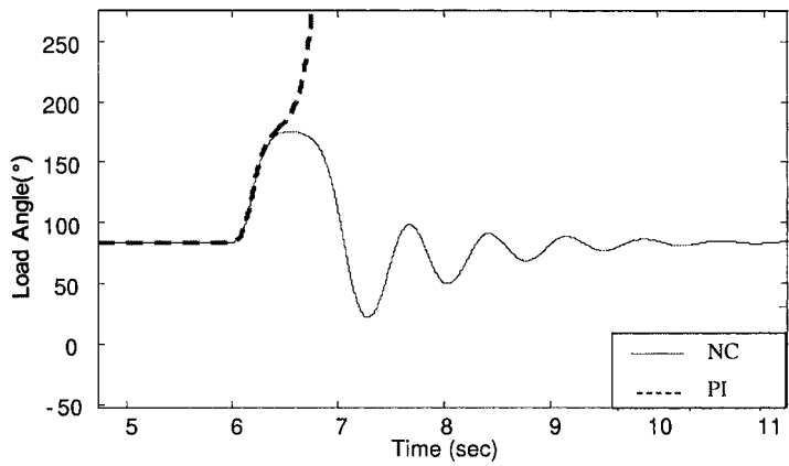
Figure 10.23. Load angle response of the synchronous generator operating ( P = 0.8 p.u. and Q = 0.15 p.u.) for a 180 ms three phase short circuit at Bus 2.
