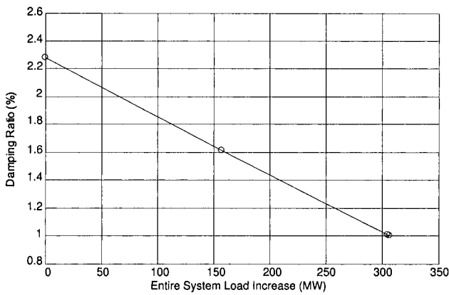
Figure 4.6. Damping ratio vs. entire system load increase.
