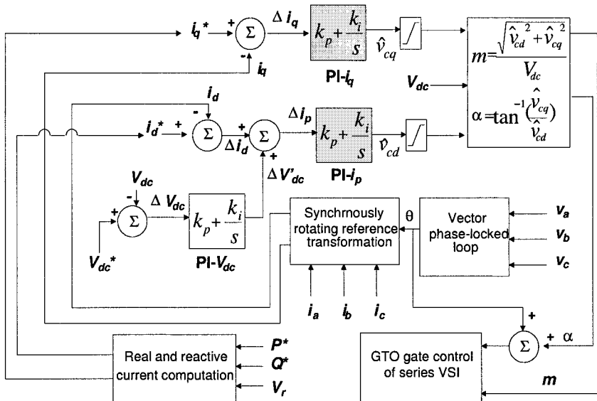
Figure 10.4. P - Q automatic power flow control diagram for the internal control of the SSSC.
