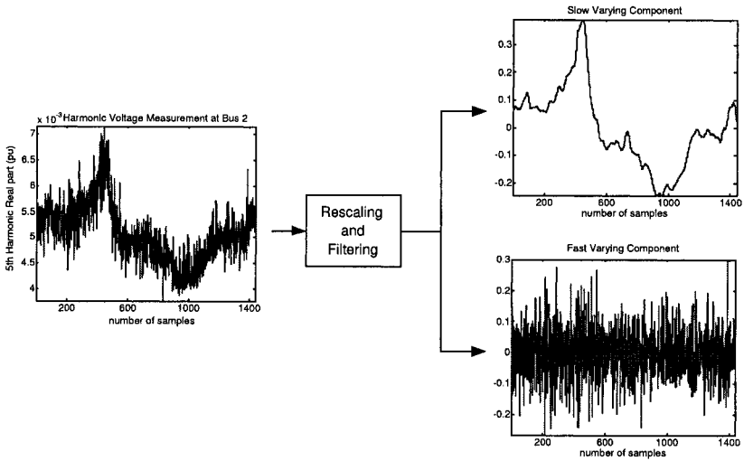
Figure 13.1. Rescaling and filtering of harmonic voltage measurements.
