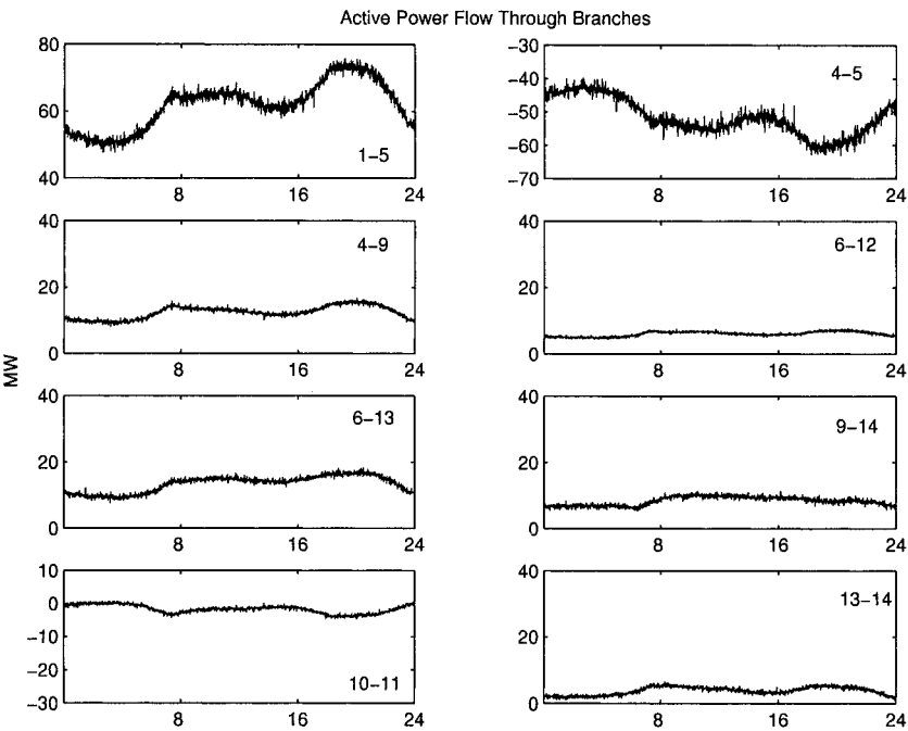
Figure 13.4. Mixed signals: Active power flow through branches.
