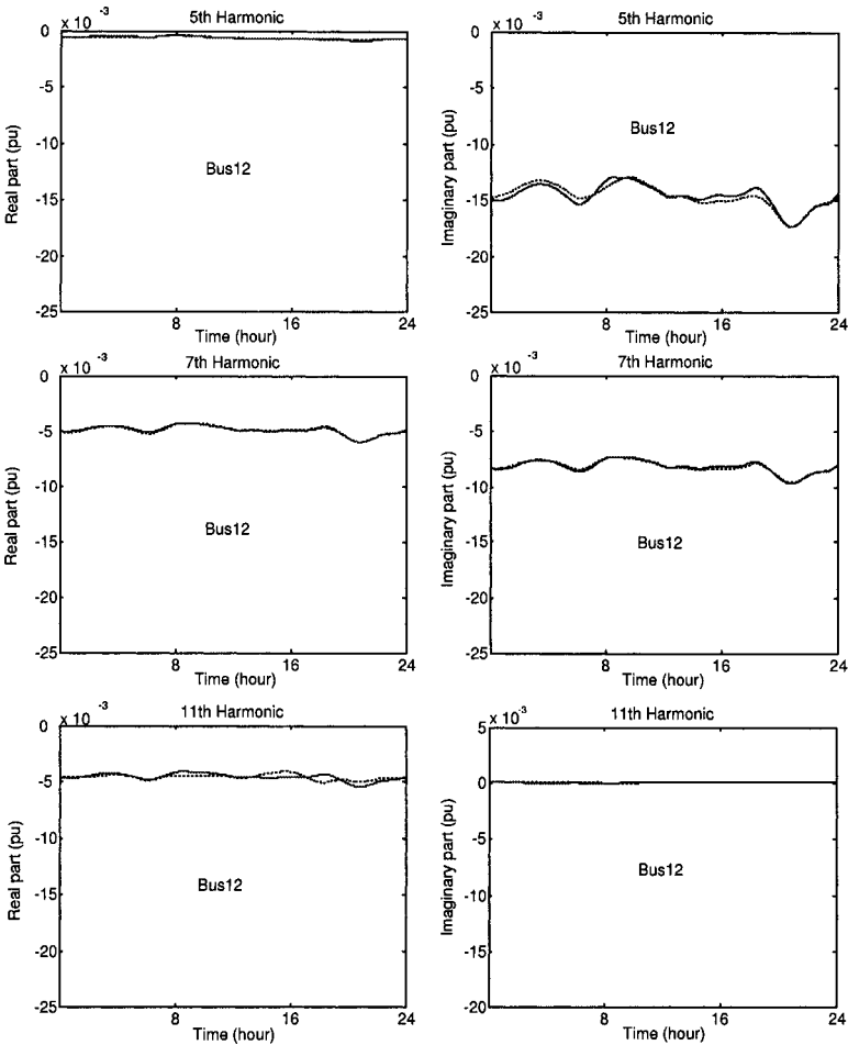
Figure 13.12. Comparison of smoothed harmonic components of current injection at Bus 12.
