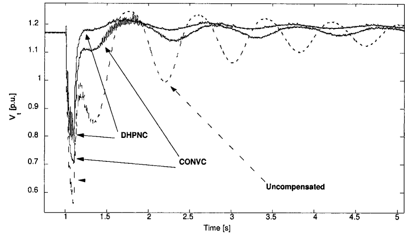
Figure 10.30. A 100 ms three phase short circuit test: V_t .
