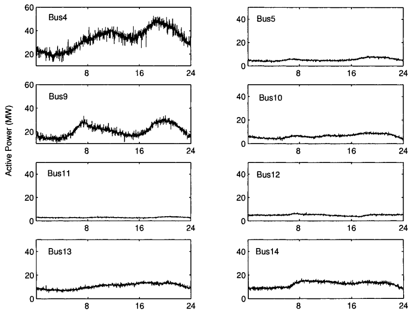
Figure 13.3. Original source signals: Active power drawn by load buses.
