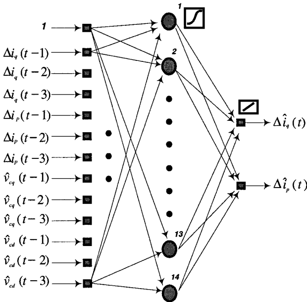
Figure 10.25. Input-output mapping of the model network at t used in the critic network adaptation in Figure 10.24.
