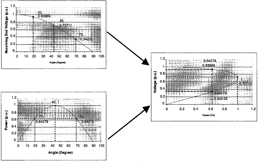
Figure 3.2. Process to develop PV curve from voltage-angle and power-angle curves.
