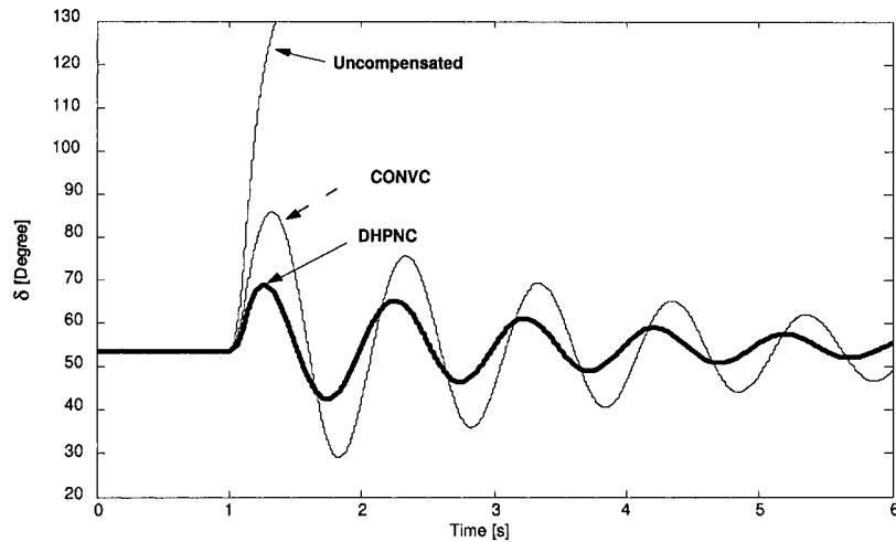
Figure 10.31. A 120 ms three phase short circuit test: \delta .
