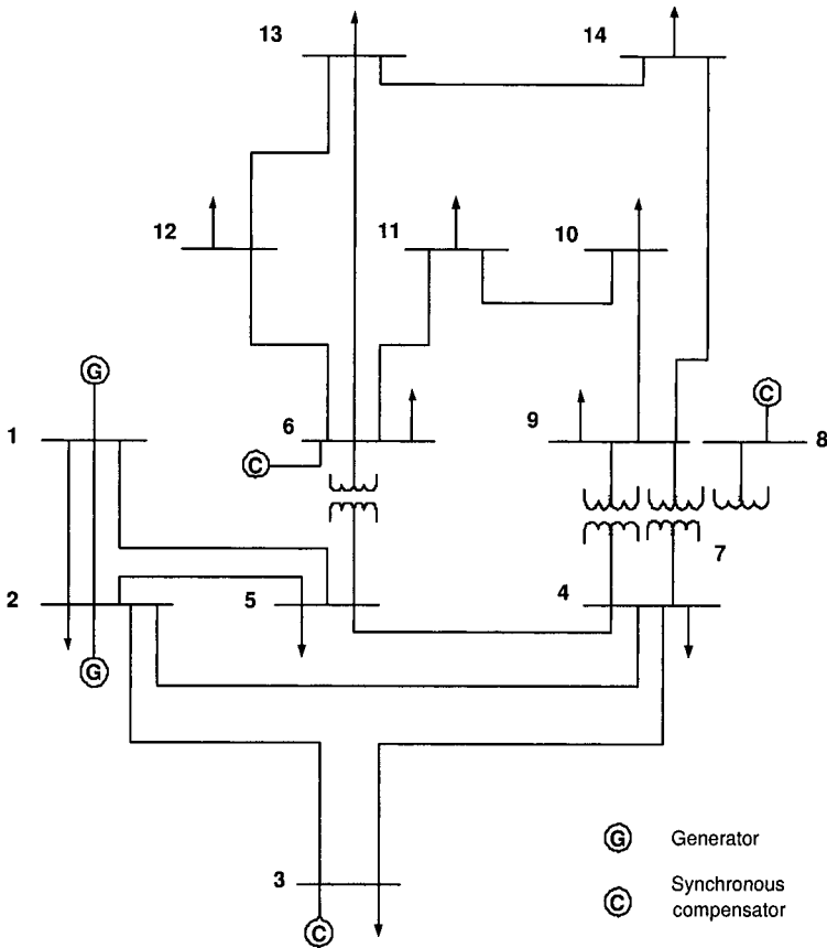
Figure 13.2. The one-line diagram of the IEEE 14-bus system.
