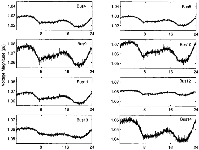
Figure 13.7. Mixed signals: Voltage magnitude measurements at load buses.
