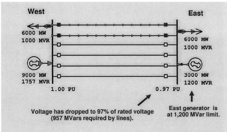
Figure 2.8. Illustration Case 5 (four lines out).
