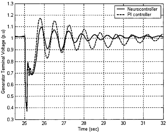
Figure 10.13. Generator terminal voltage during a 100 ms short circuit at the midline.
