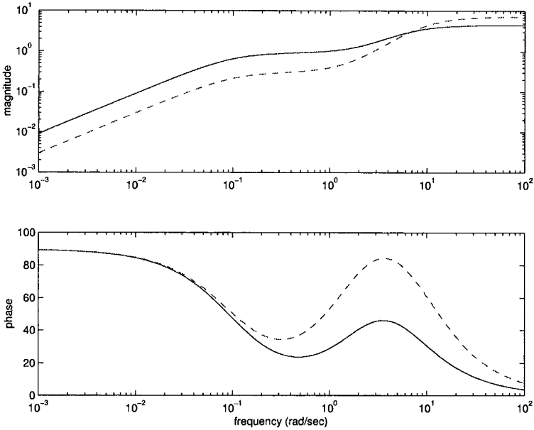
Figure 11.12. Frequency response of the nominal SVC POD controller (dashed line) and the GA-designed SVC POD controller (solid line).
