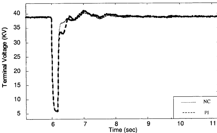
Figure 10.21. Terminal voltage response of the synchronous generator operating ( P = 0.65 p.u. and Q = 0.12 p.u.) for a 180 ms three phase short circuit at Bus 2.
