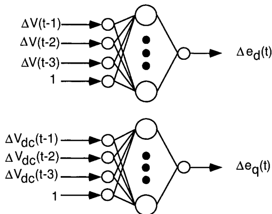
Figure 10.11. Neurocontroller structure for a STATCOM.
