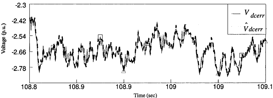
Figure 10.20. Actual signal V_{err}(t) of the plant and estimated signal \hat{V}_{err}(t) by the SHNI.
