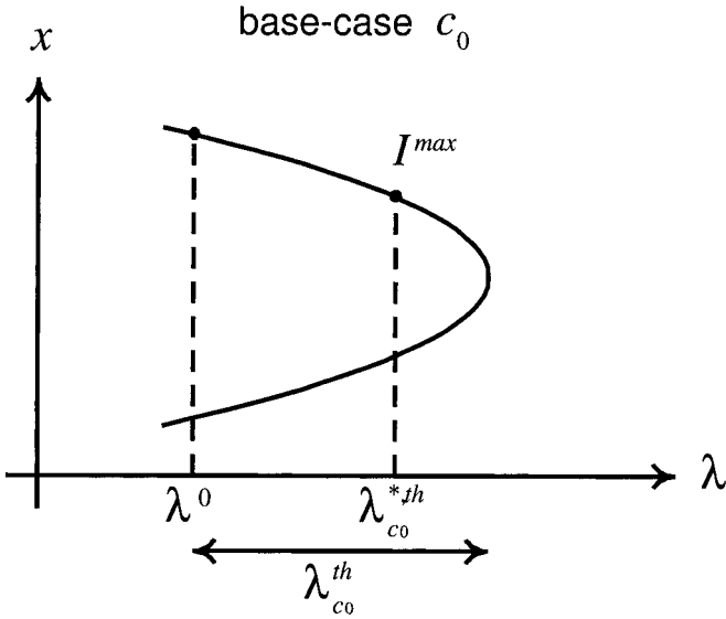
Figure 5.5. The thermal-limit load margin \lambda_{C_0}^{th} for the base case power system C_0 .
