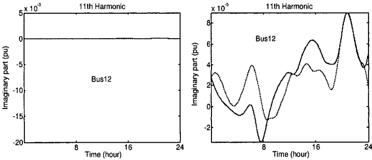
Figure 13.13. Imaginary part of the 11 th harmonic source current at Bus 12 at scale 10^{-3} and scale 10^{-5} .
