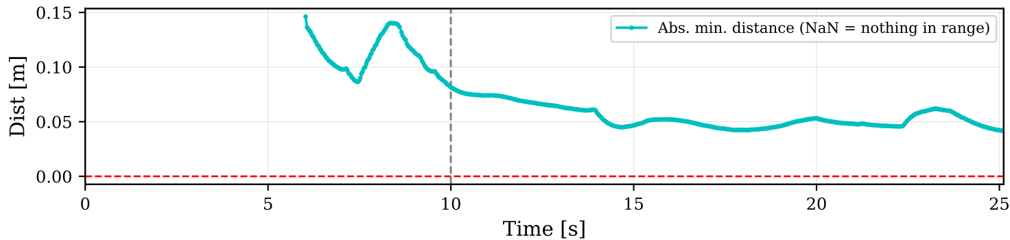
Absolute Minimum Collision Distance
