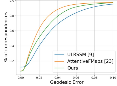
Figure 6. PCK curves on the SMAL dataset
