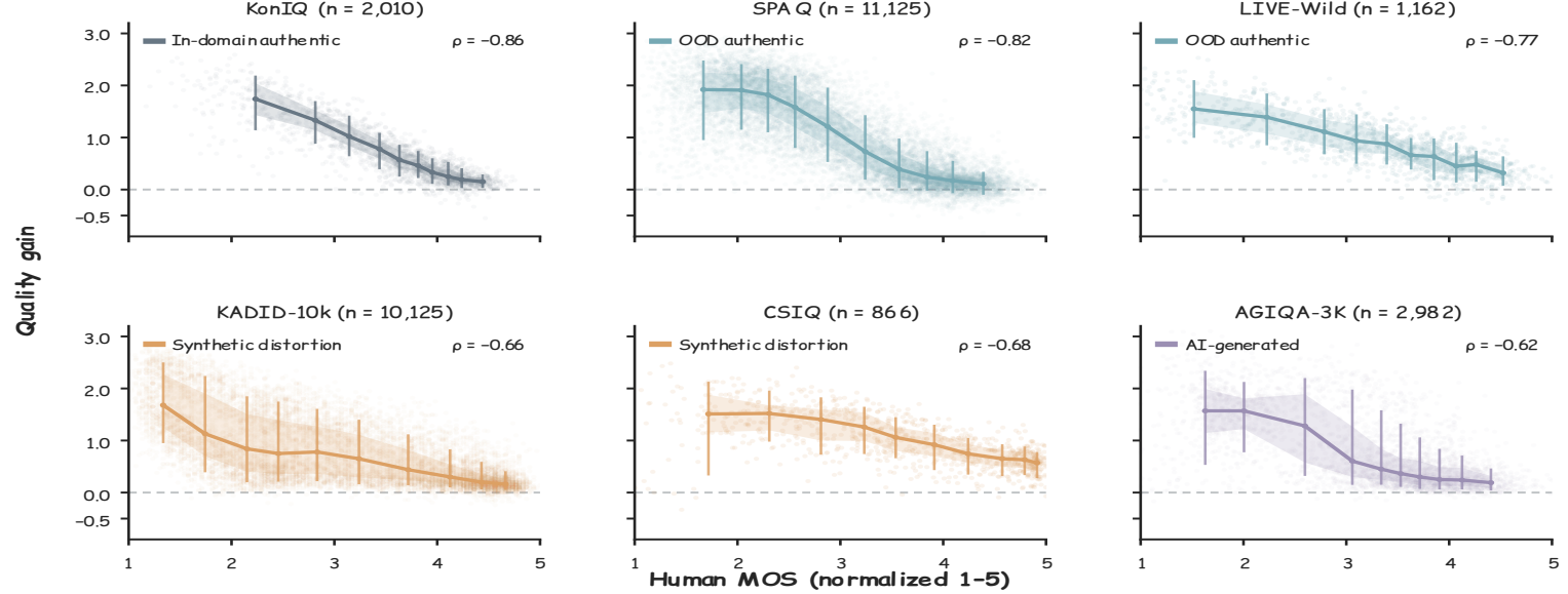
(a). Quality Gains vs. MOS
