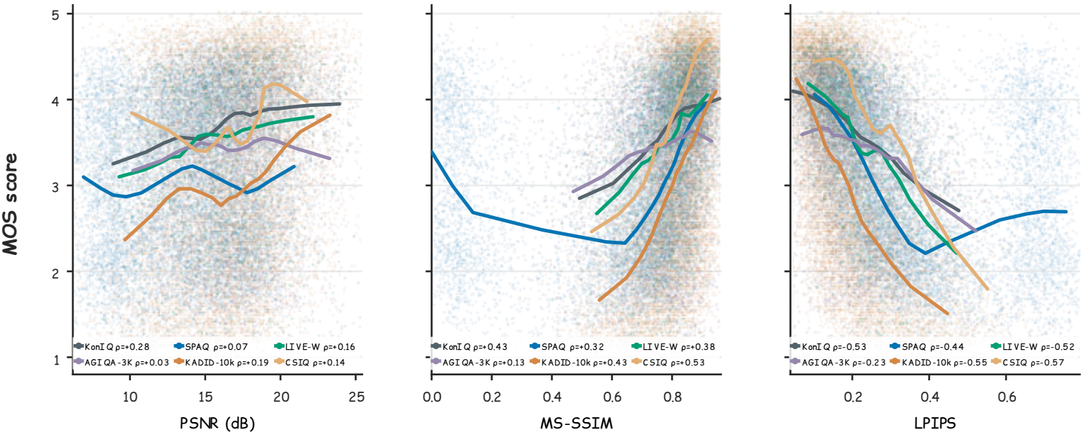
(c). MOS vs. Reference Metrics
