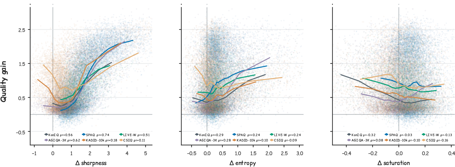
(b). Quality Gains vs. Low-level feature
