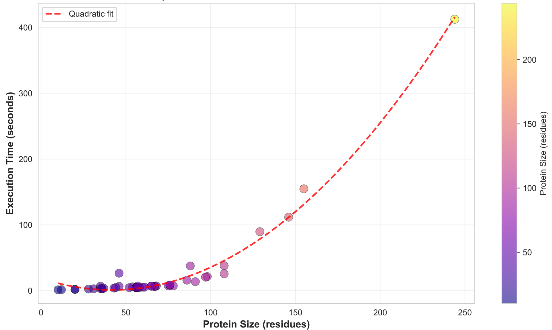
Computational Performance vs Protein Size
