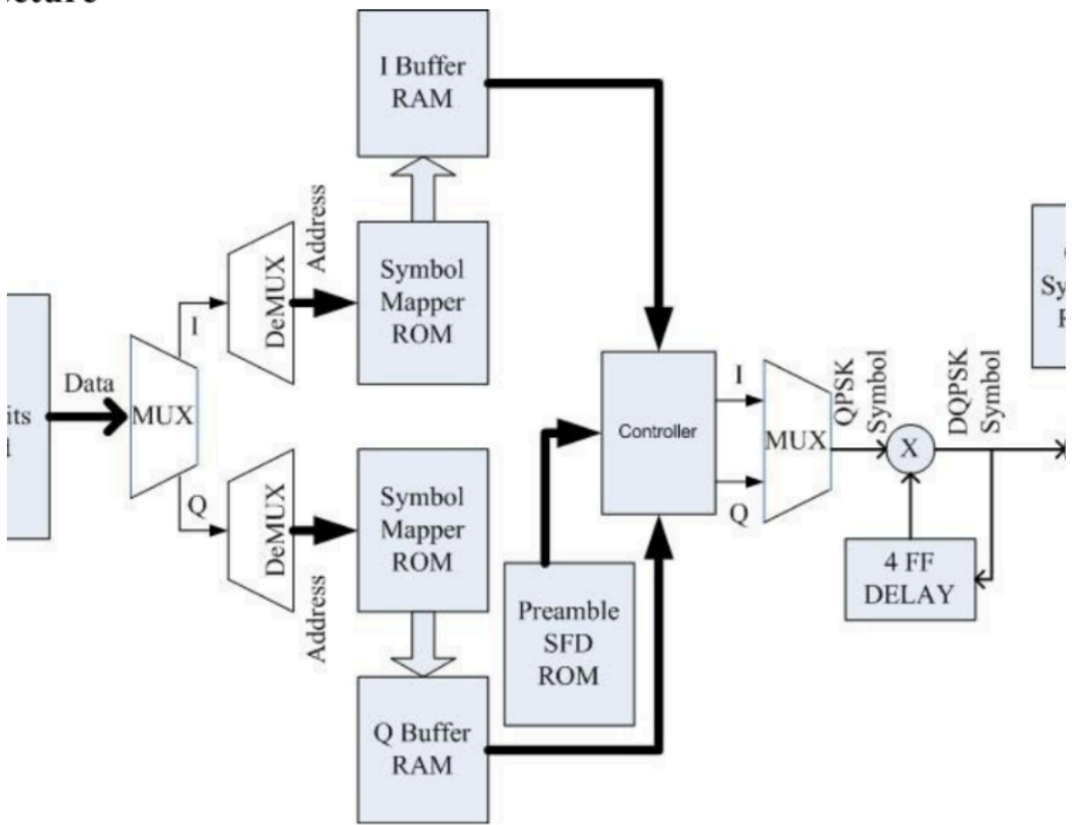
Figure 3-3, CSS transmitter architecture
