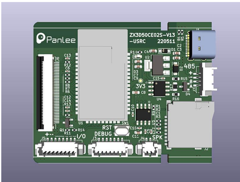
Fig.1 Hardware Interface
