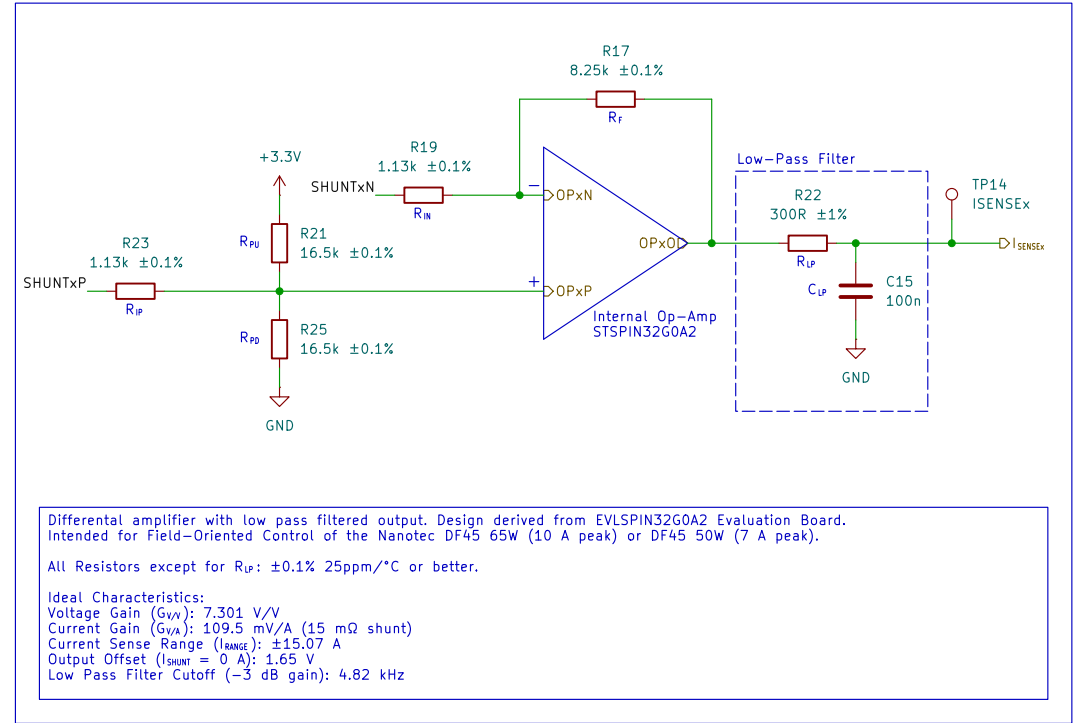
Current Sensing Op-Amp with Low Pass Filtered Output
