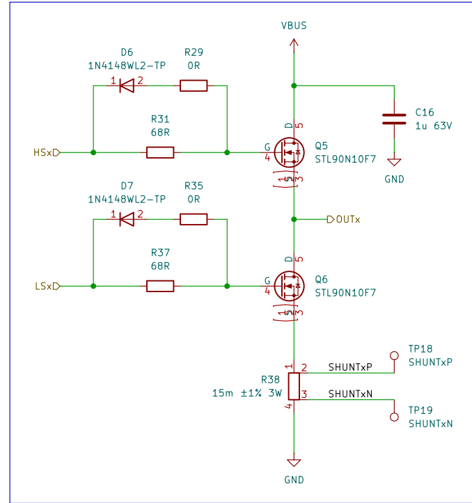
Half Bridge for BLDC Motor Phase
