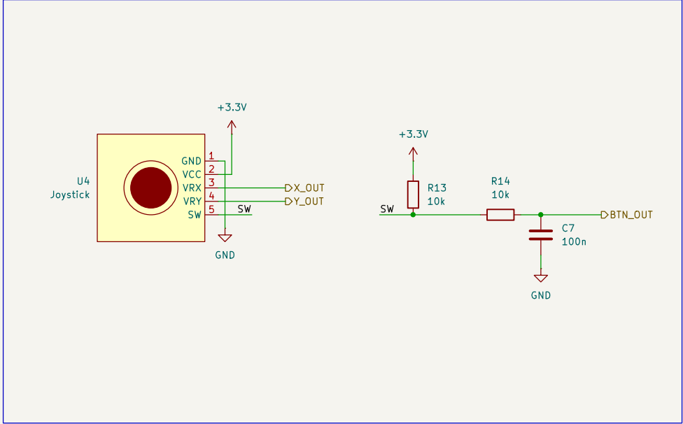
Analog Joystick with Debounced Pushbutton
