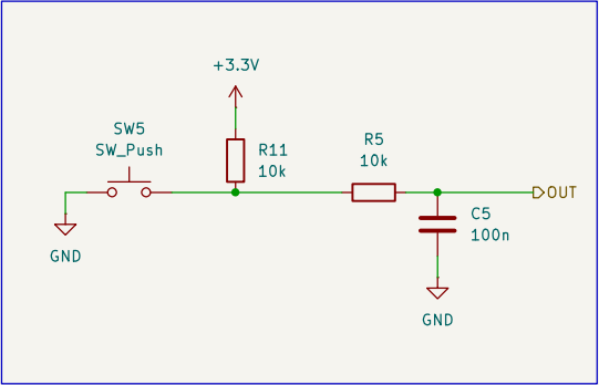
Debounced Pushbutton, RC Filter
