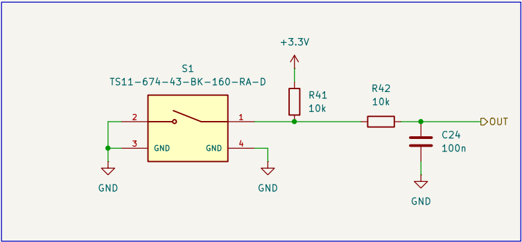
Debounced Right Angled Pushbutton, RC Filter
