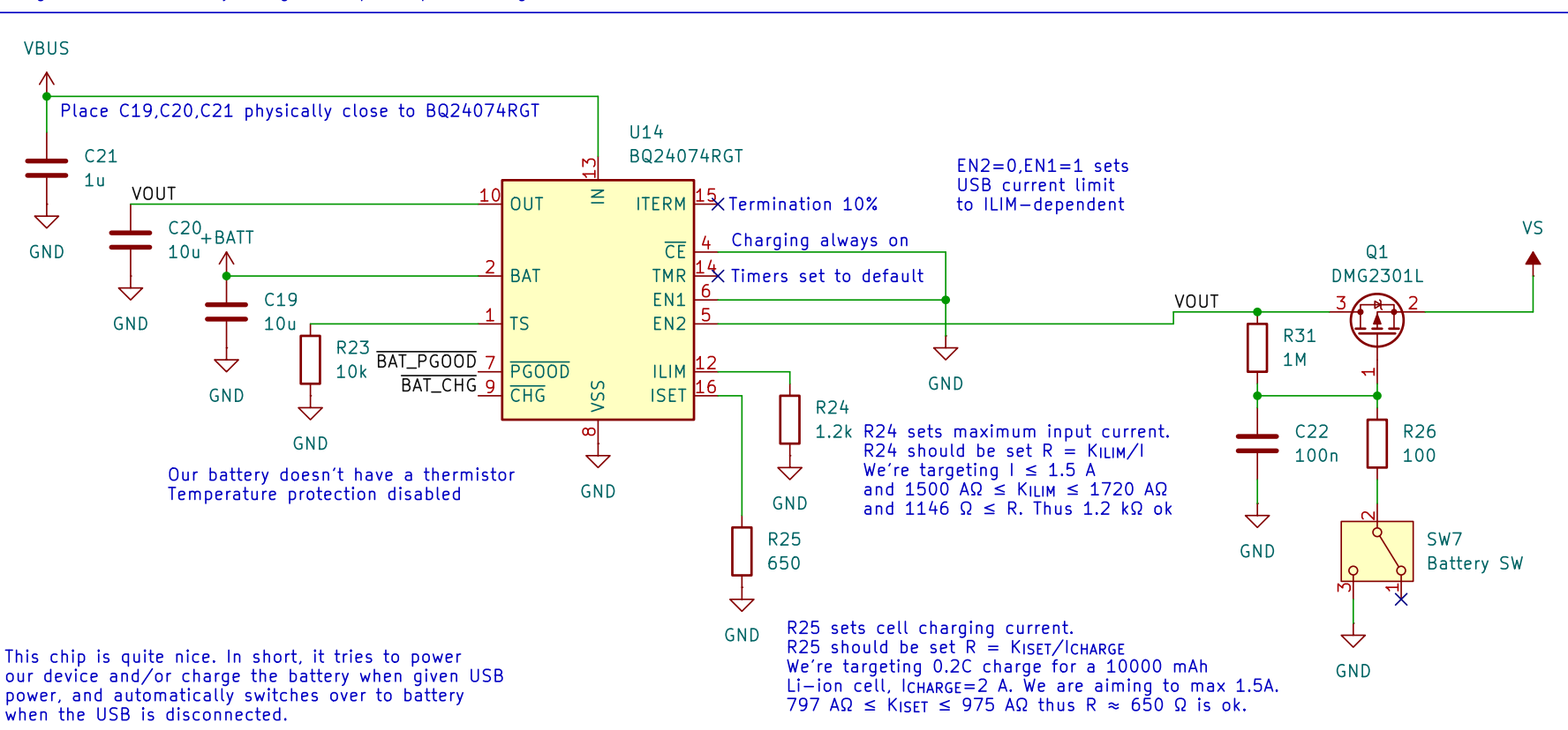
Integrated Li-ion battery charger and power path management
