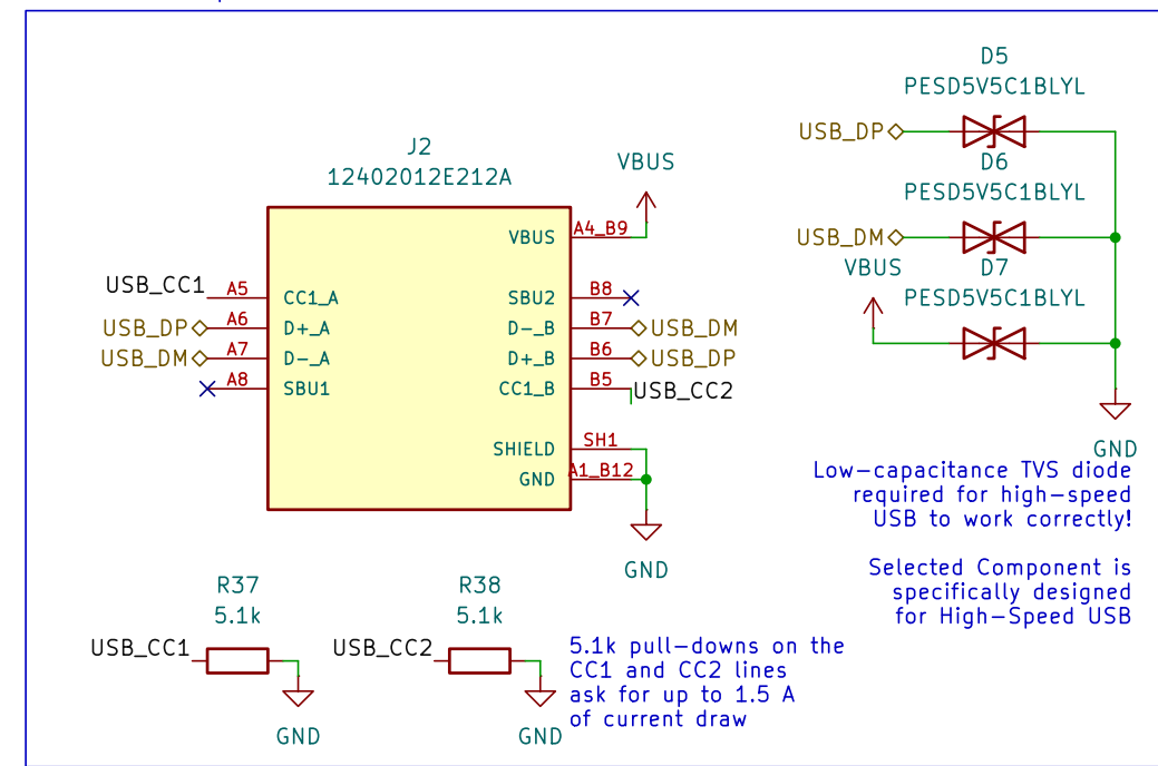
USB C Data + Up to 1.5A Power with ESD Protection
