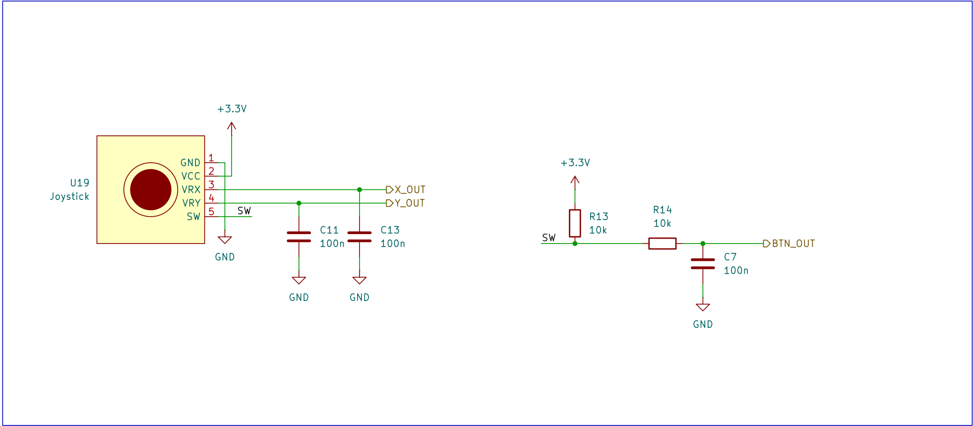
Analog Joystick with Debounced Pushbutton
