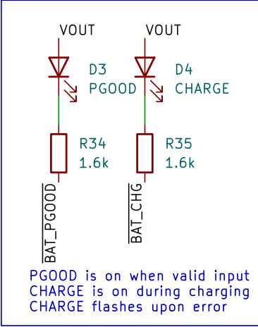
Indicator LEDs
