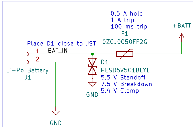
JST-PH Battery Terminal w/ ESD. Overcurrent Protection
