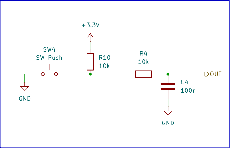
Debounced Pushbutton, RC Filter
