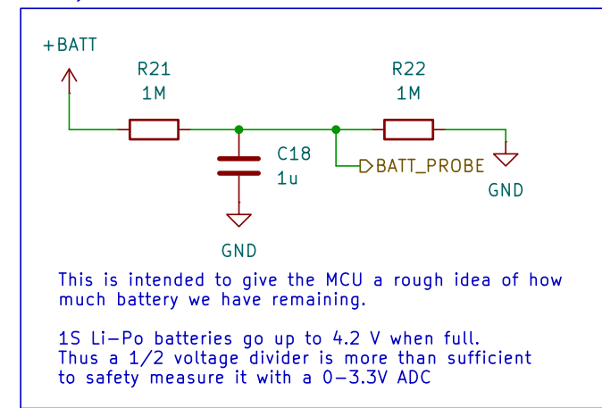
Battery Probe
