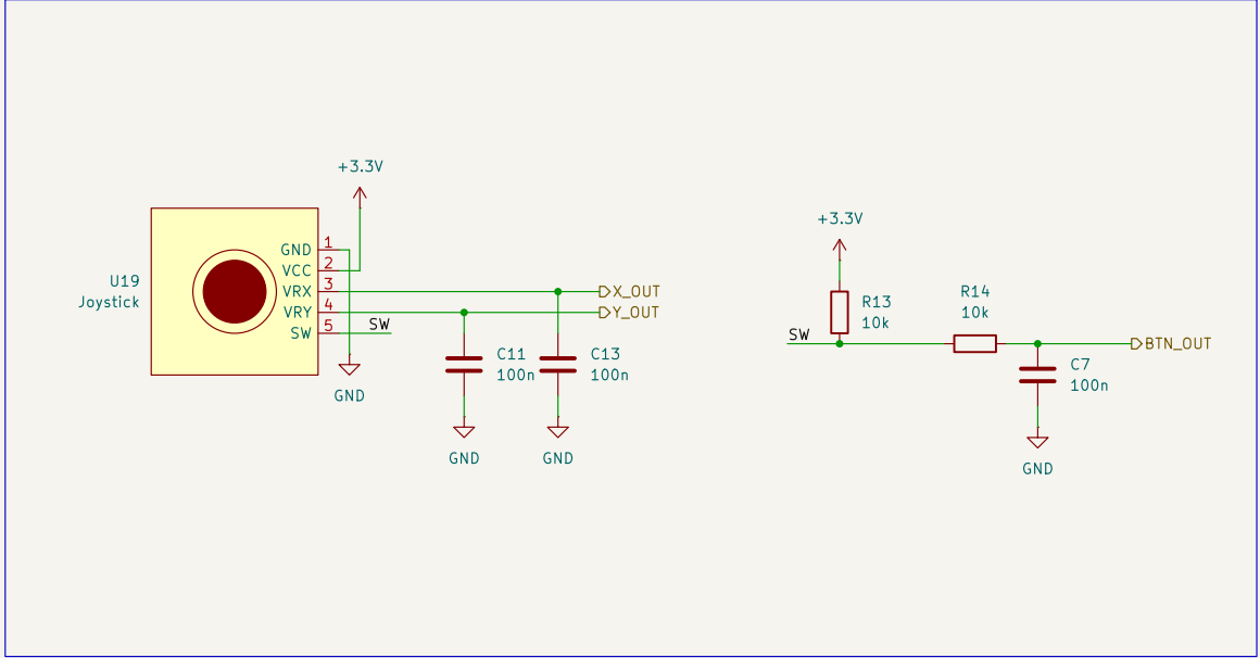
Analog Joystick with Debounced Pushbutton
