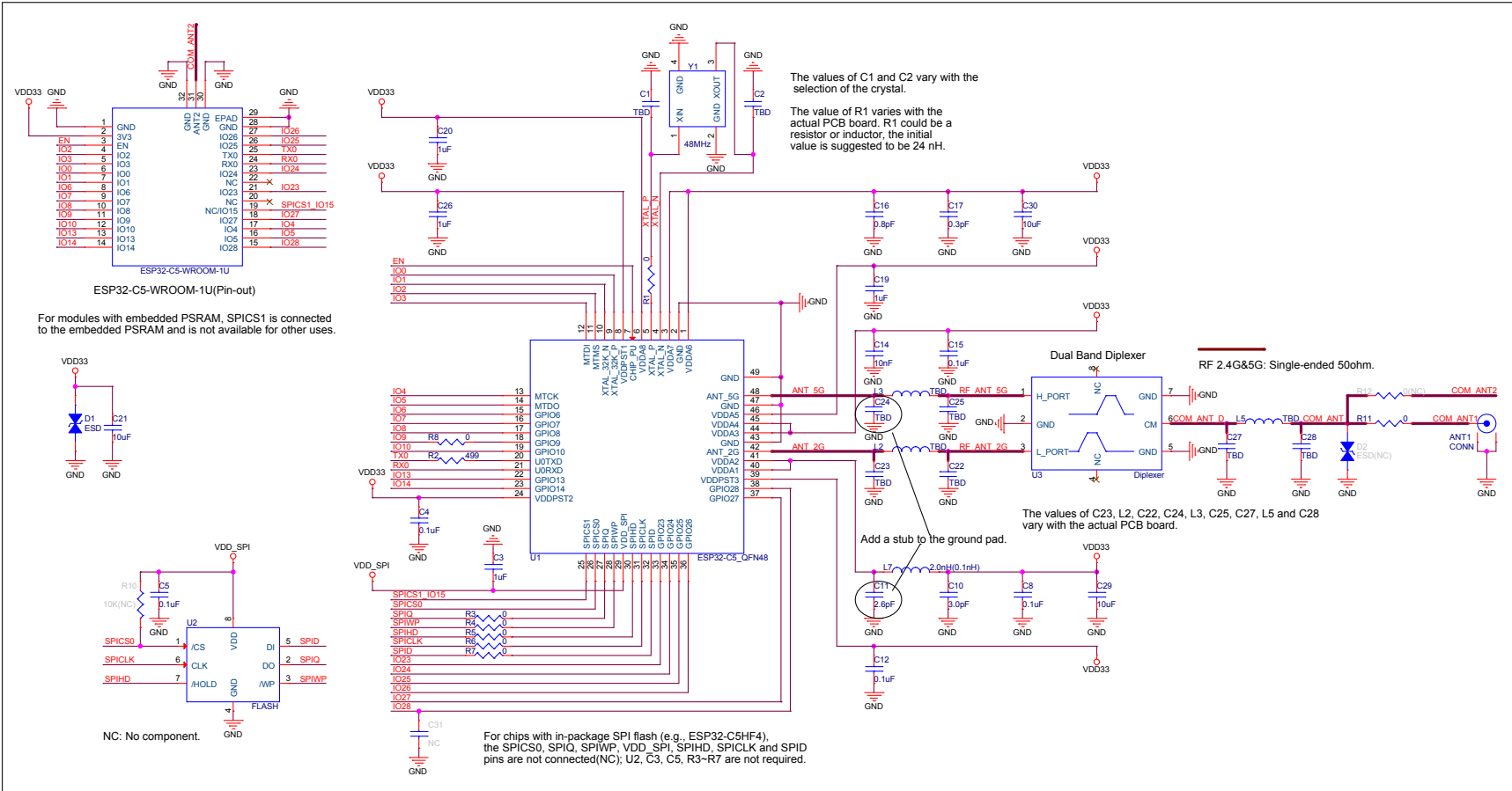
Figure 8-2. ESP32-C5-WROOM-1U Schematics
