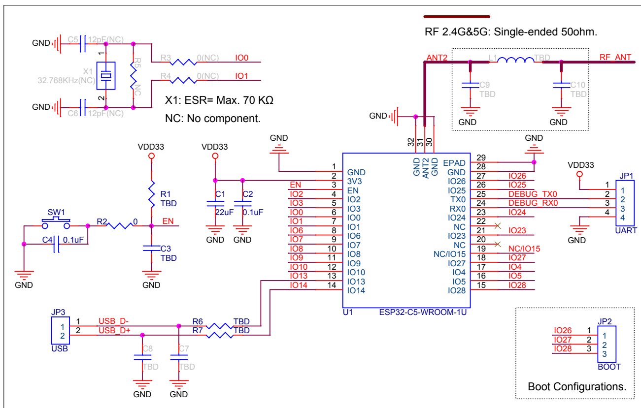
Figure 9-2. ESP32-C5-WROOM-1U Schematics
