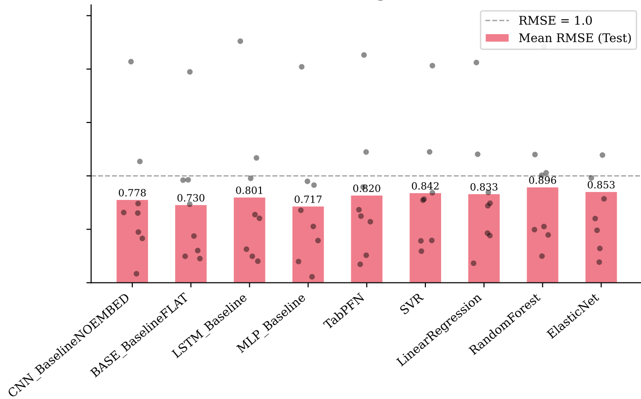
Test Split
