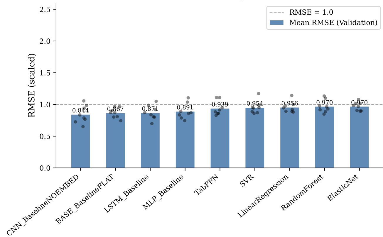
Validation Split
