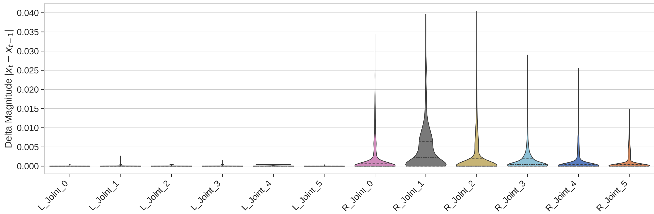
Expert Demonstrations: 1-Step Delta (Velocity) Distribution
