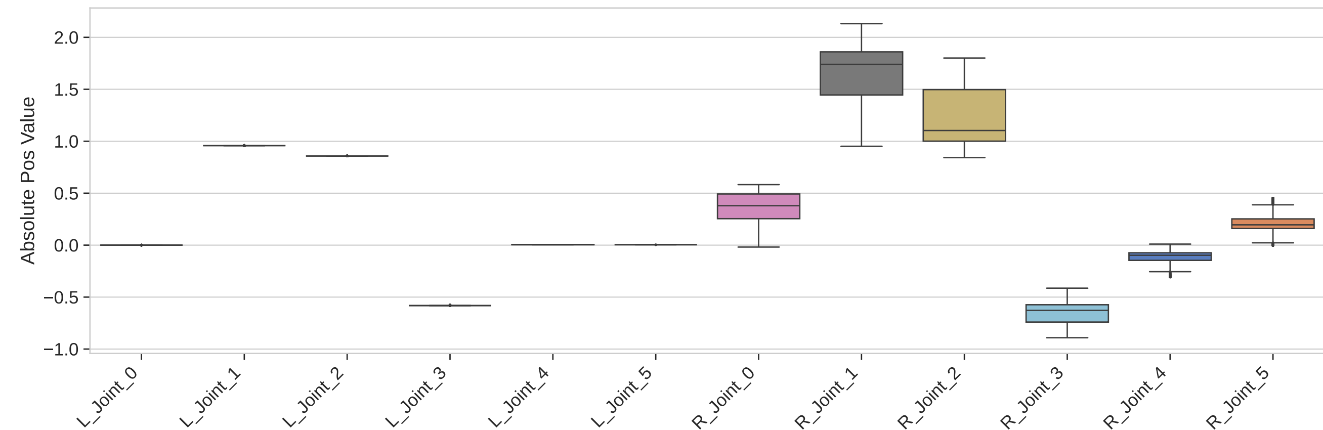
Expert Demonstrations: Absolute Position Distribution
