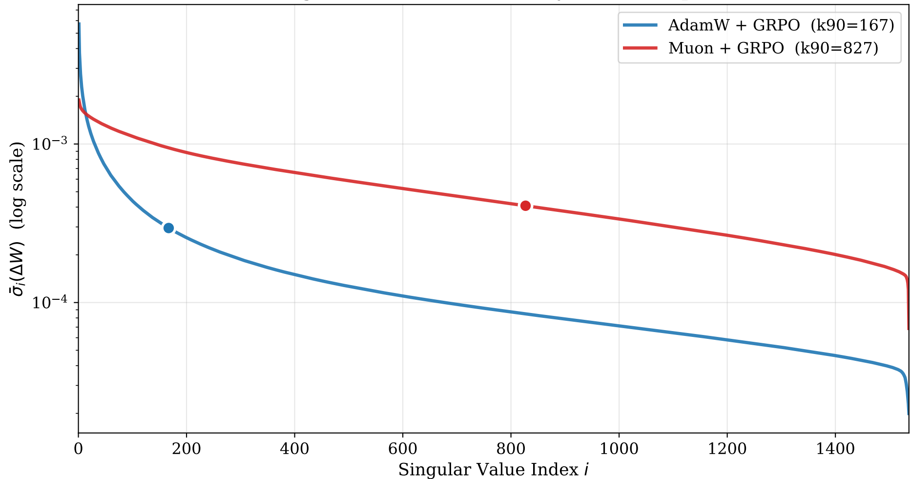
Mean Spectral Decay of \Delta W = W_{exp} - W_{base} ( \bar{\sigma}_i averaged over all transformer layers and components)
