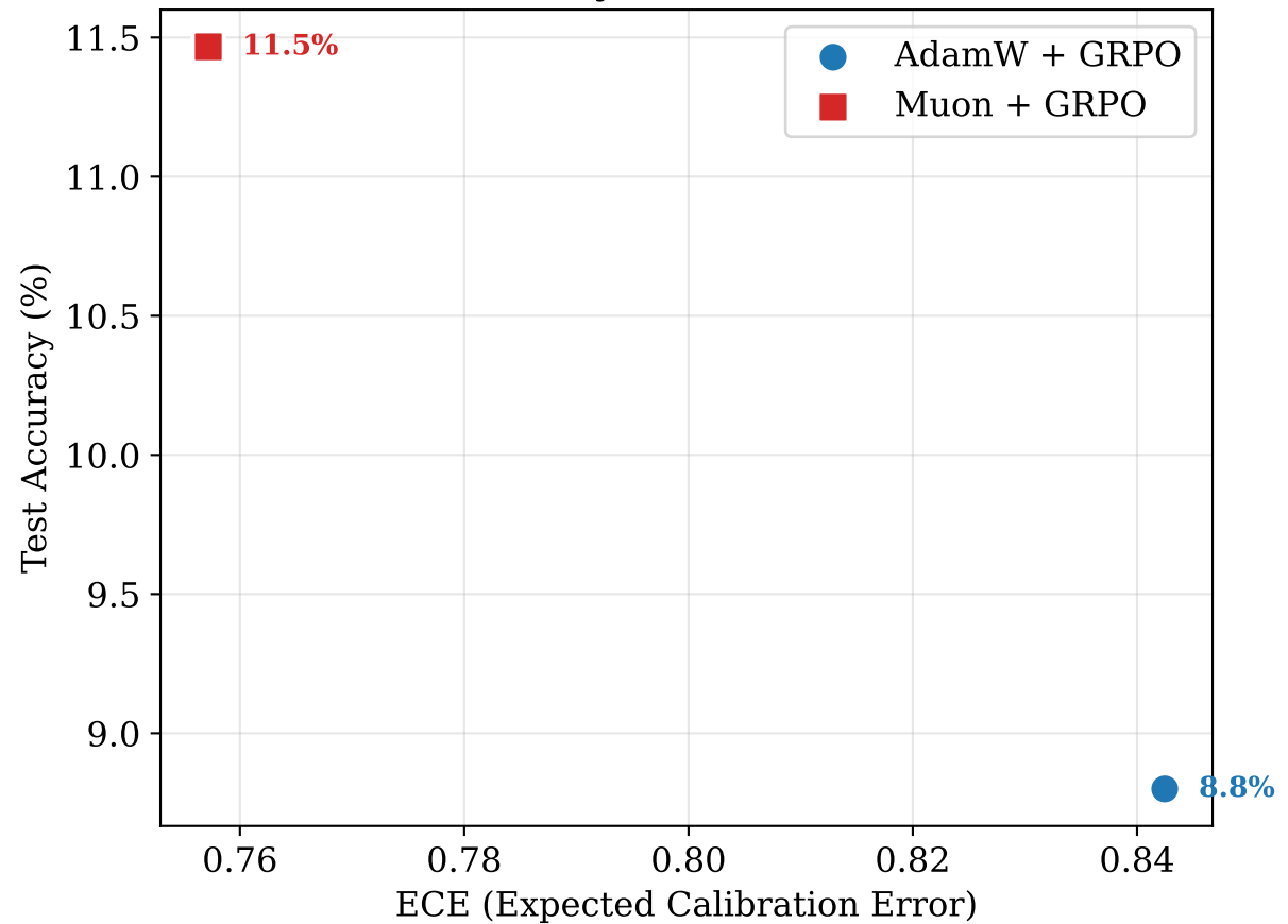
Test Accuracy vs Calibration Error
