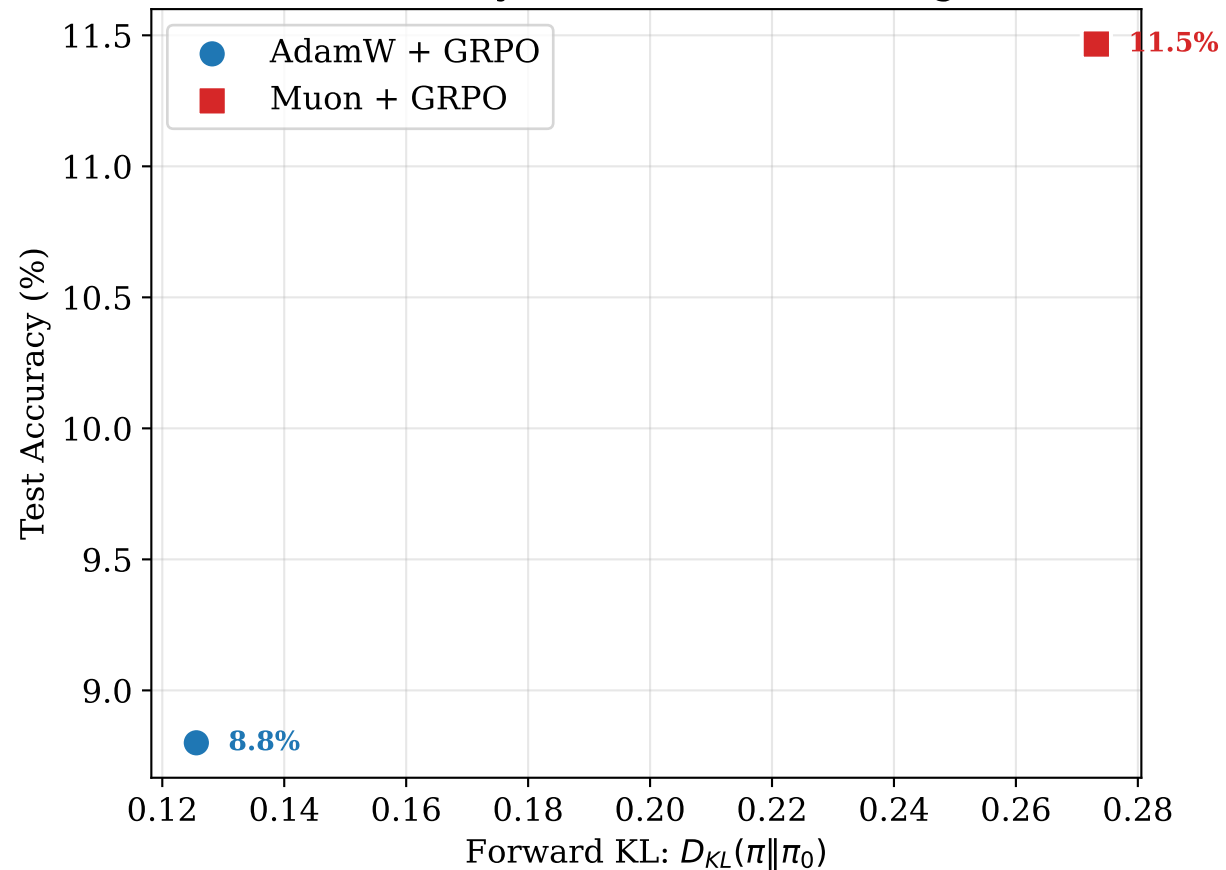
Test Accuracy vs Forward KL Divergence
