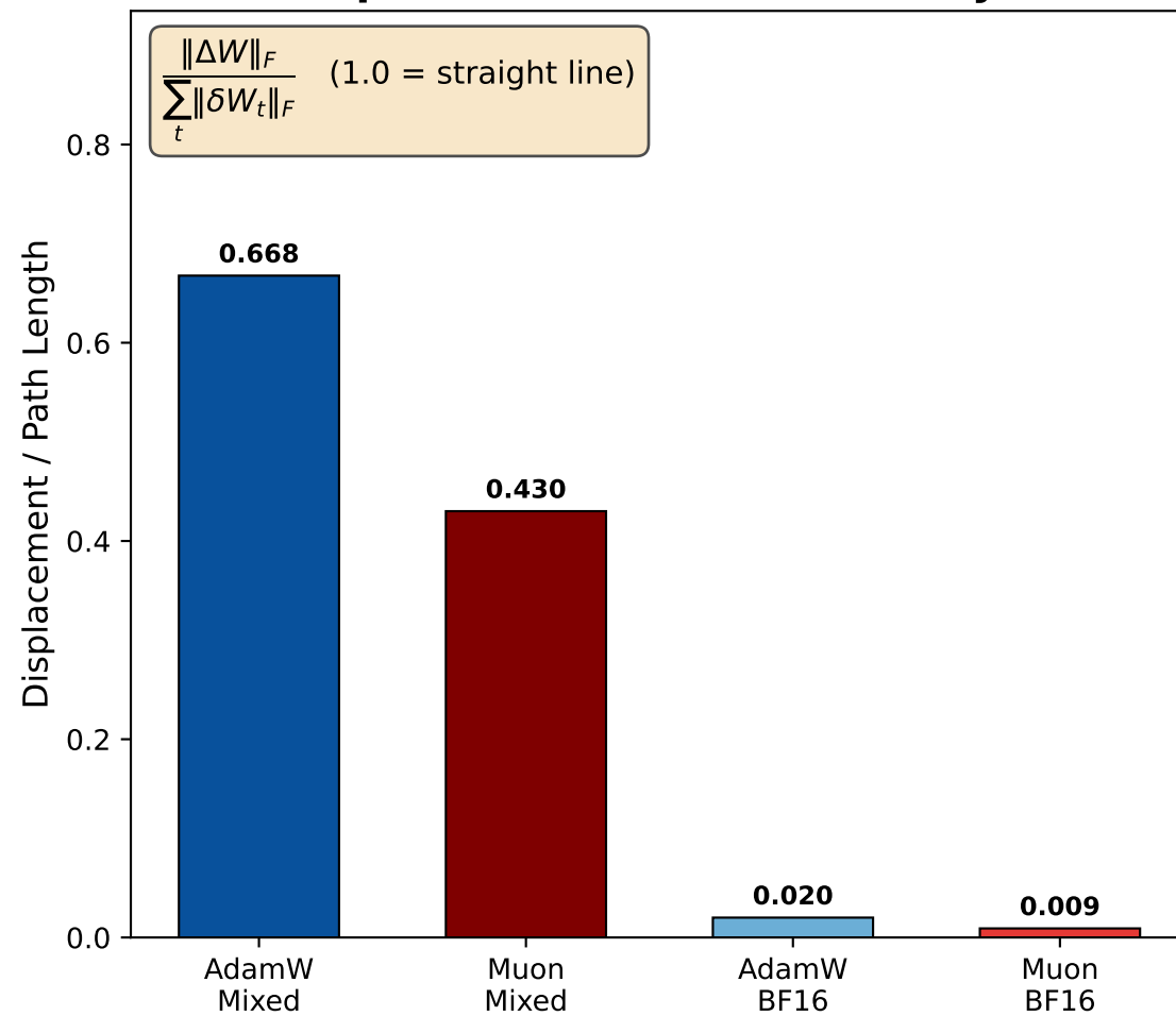
Optimization Path Efficiency
