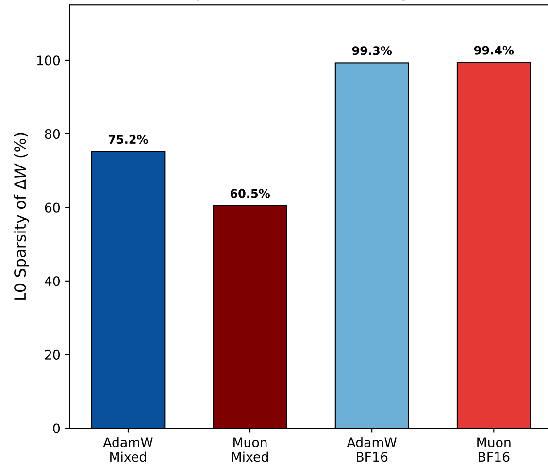
Weight Update Sparsity ( \Delta W )
