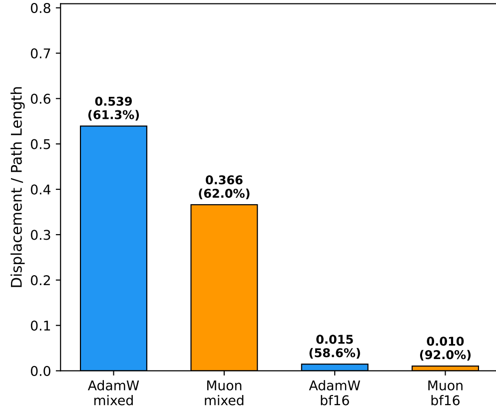
Path Efficiency (1.0 = straight line)
