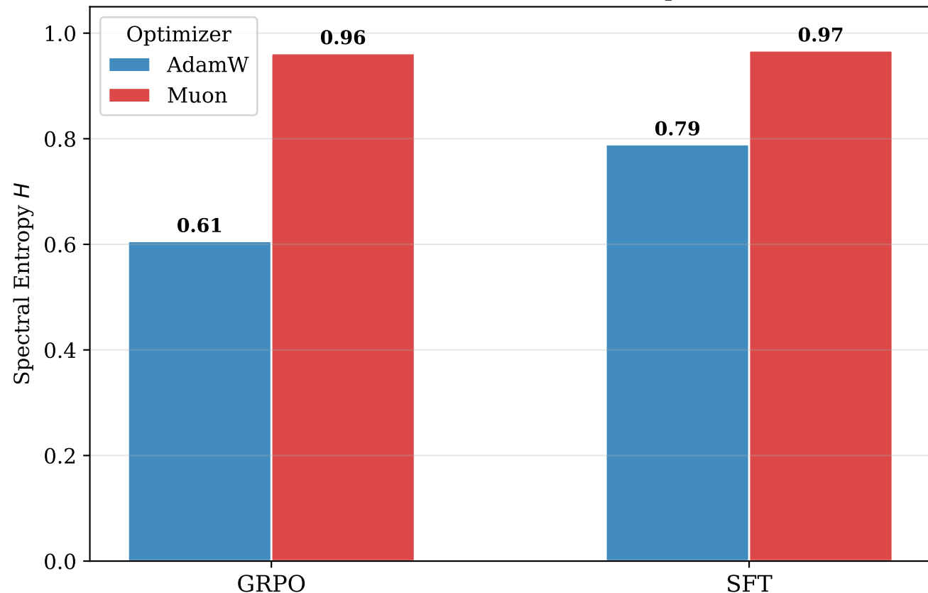
Spectral Entropy (FP32 Only) Lower = more concentrated update
