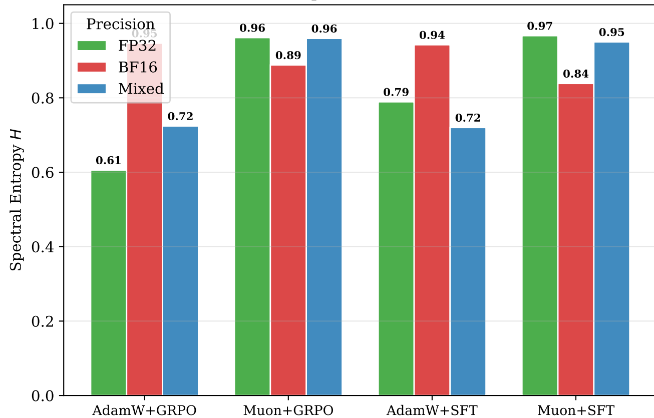
Spectral Entropy Across Precision Modes
