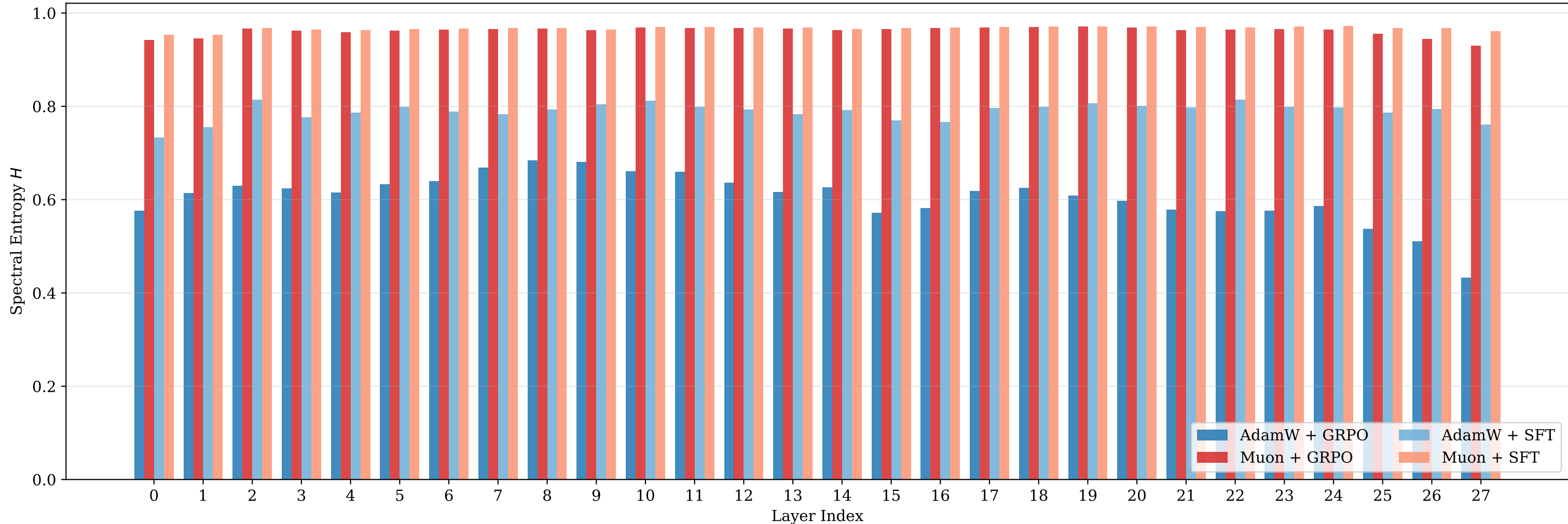
Spectral Entropy by Layer (FP32 Training) H \in [0, 1] : lower = more energy concentrated in top SVs
