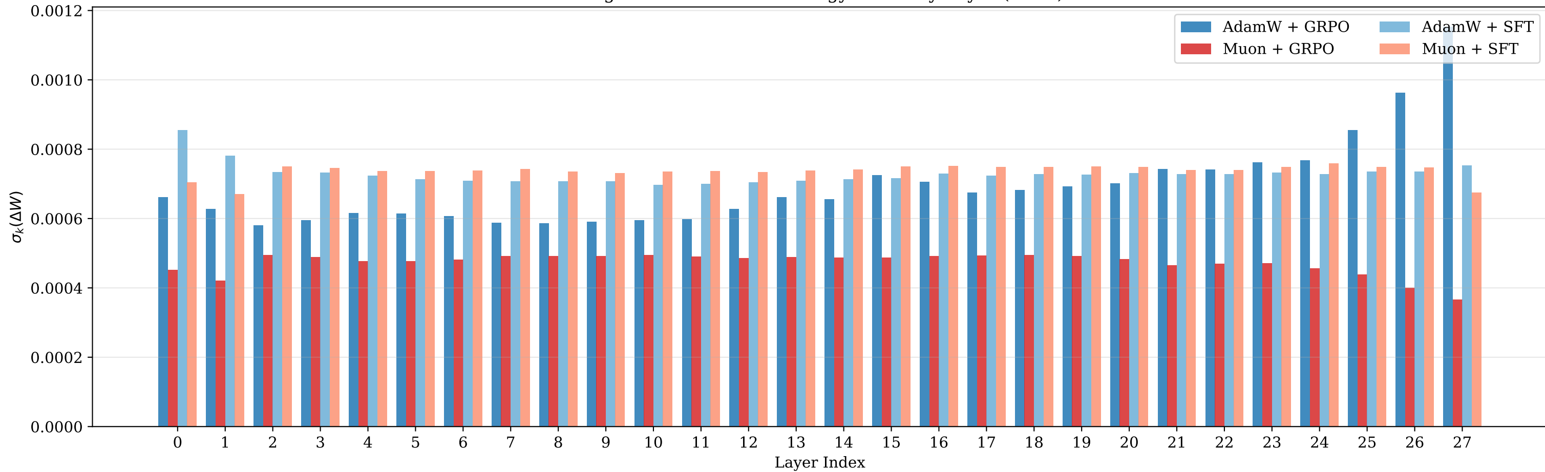
Singular Value at 90% Energy Cutoff by Layer (FP32)
