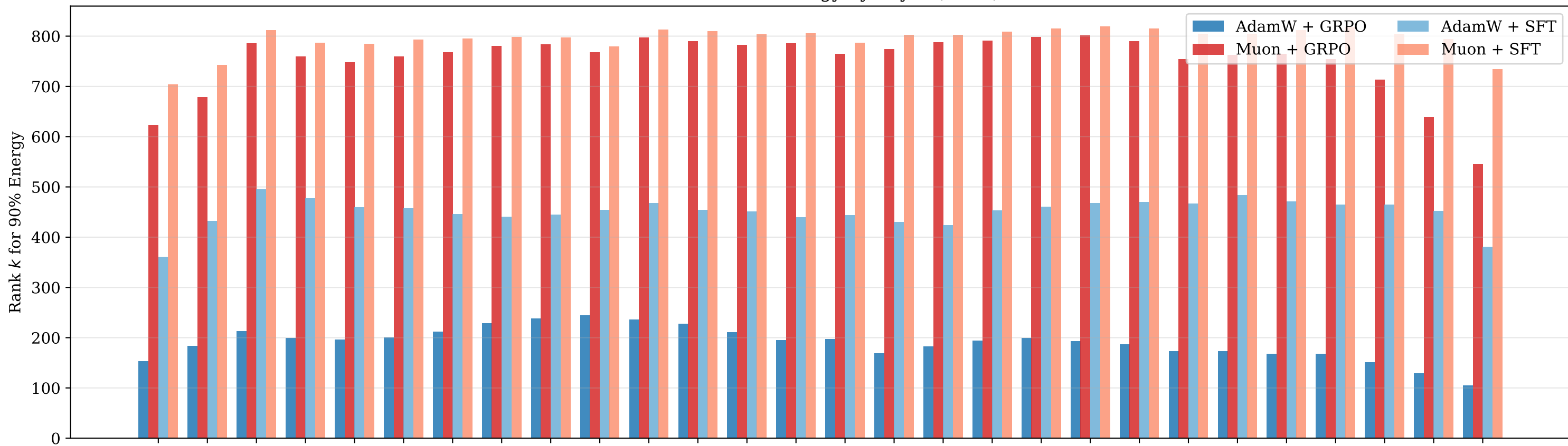
Singular Value at 90% Energy Cutoff by Layer (FP32)
