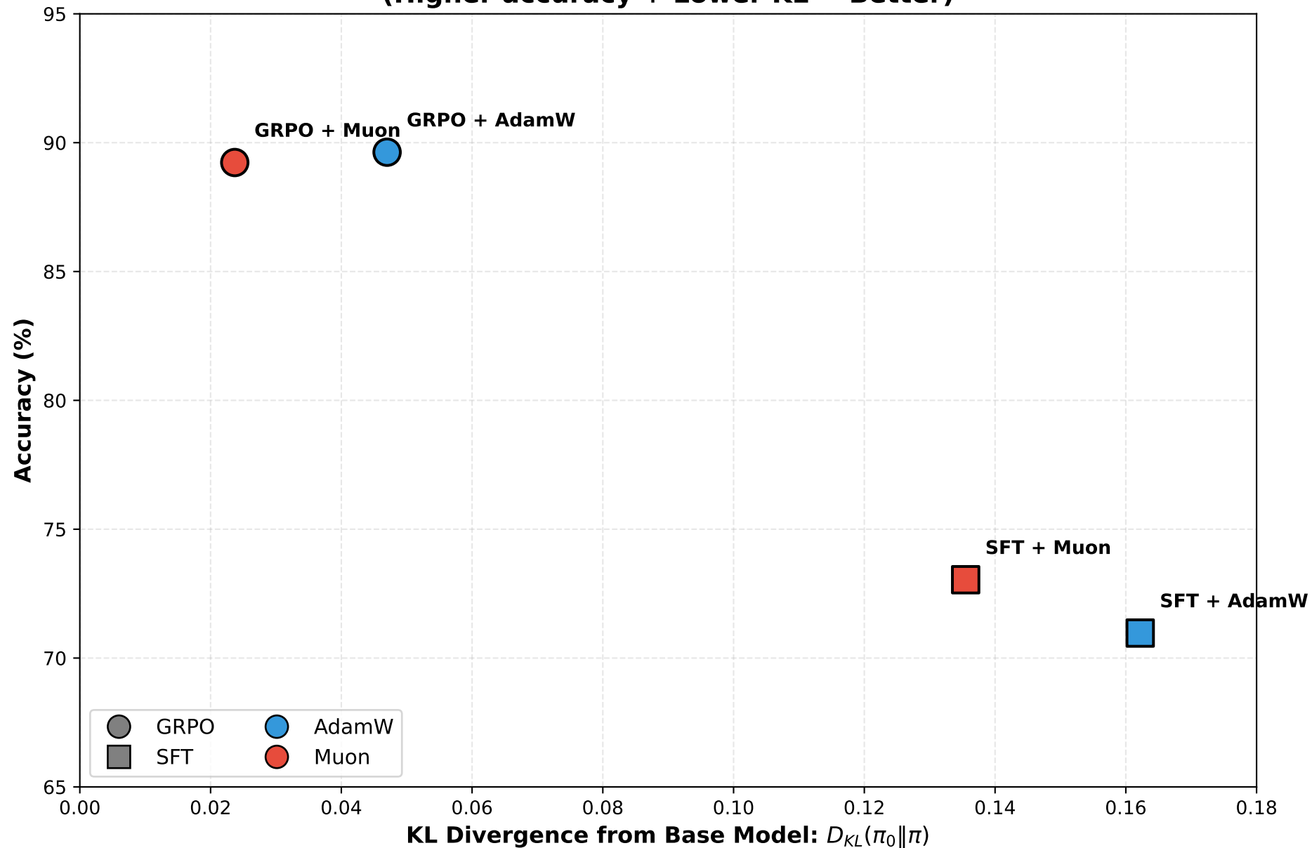
GSM8K Accuracy vs. KL Divergence (Higher accuracy + Lower KL = Better)
