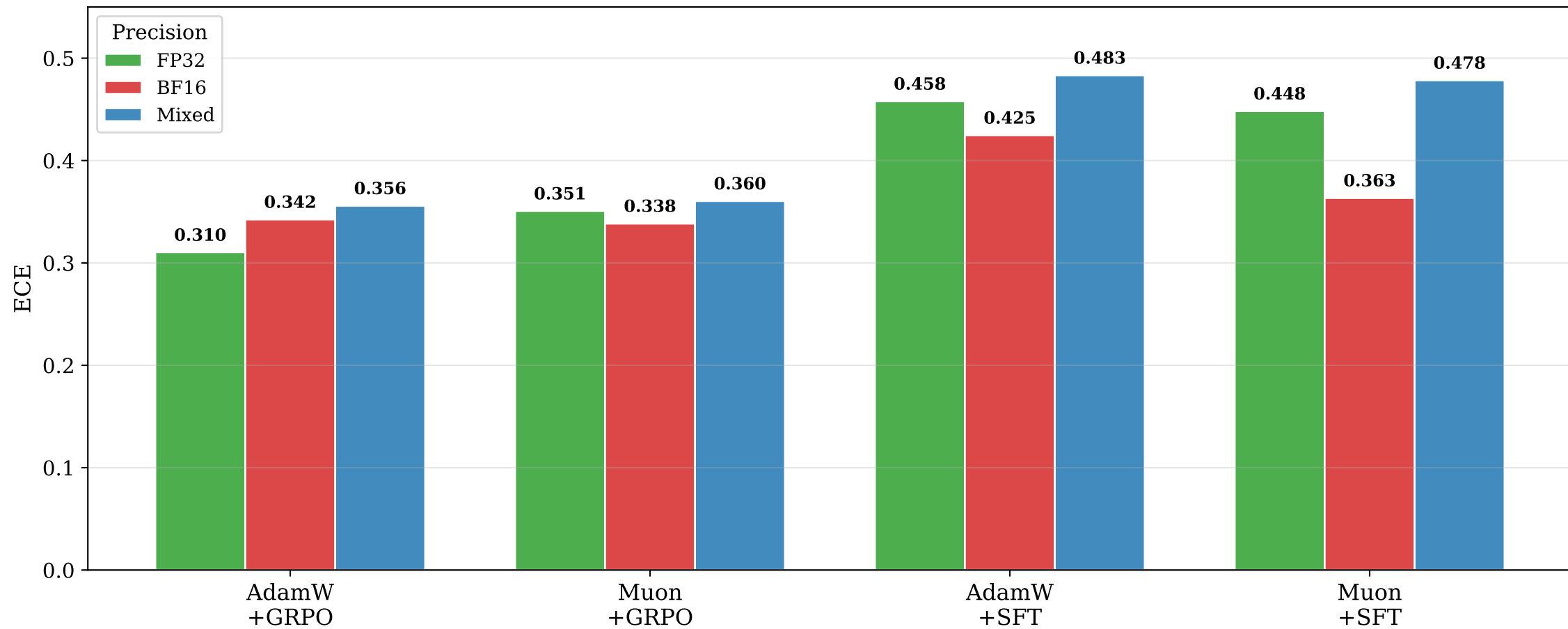
Expected Calibration Error (ECE) Across Precision Modes (FP32 logprobs, greedy decoding, confidence = answer content tokens)
