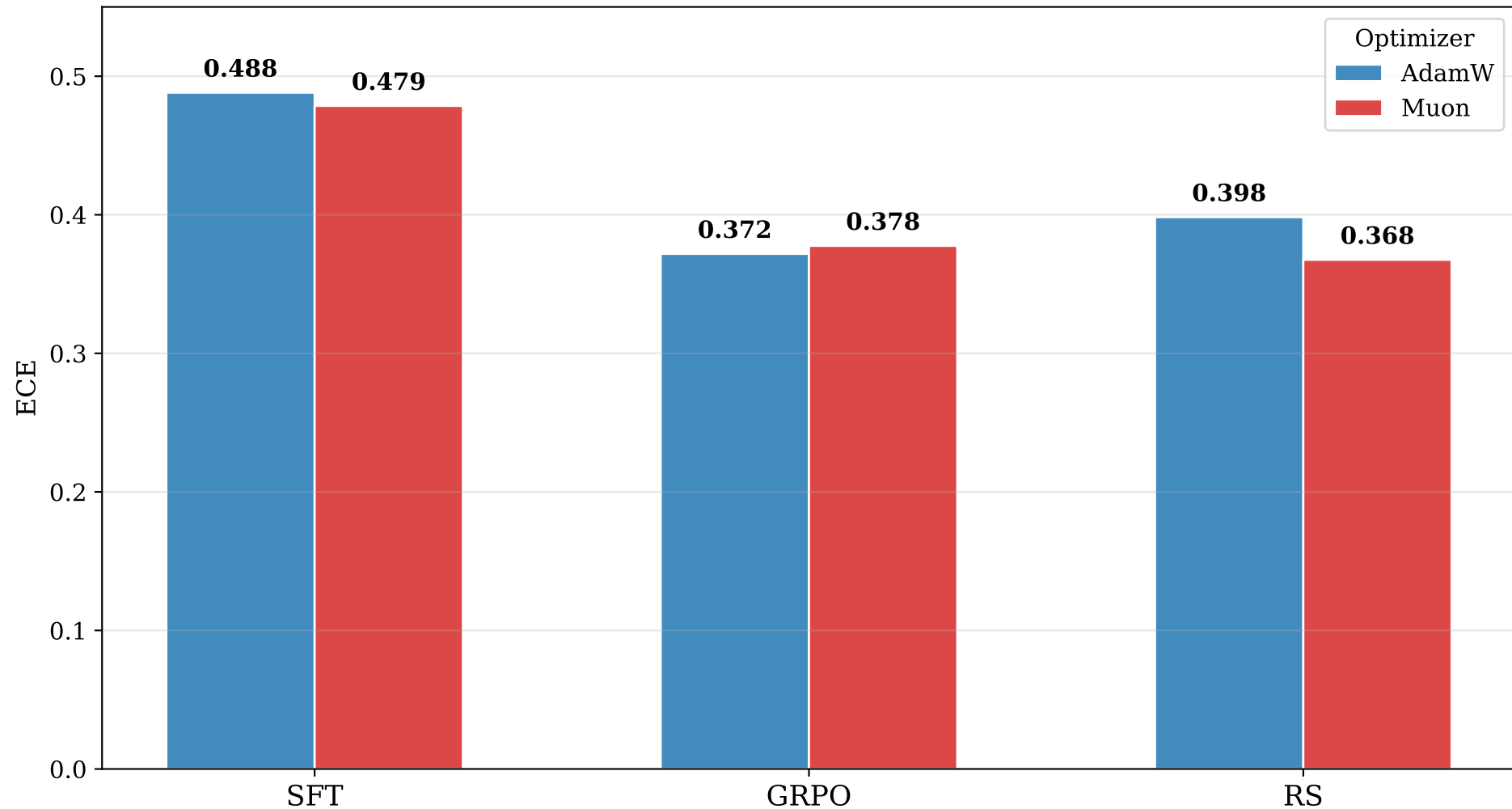
Expected Calibration Error by Training Objective (~1.1M tokens, FP32 logprobs, greedy decoding)
