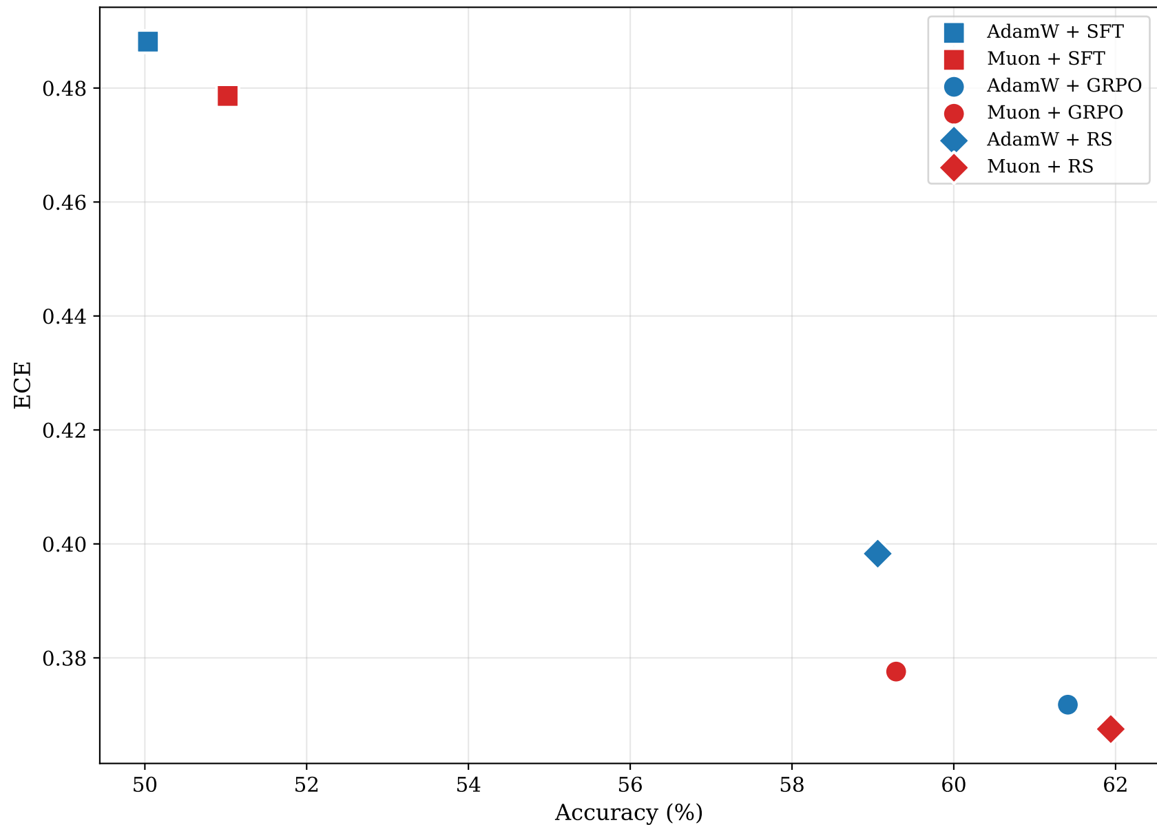
Accuracy vs Calibration Error (circle = GRPO, square = SFT, diamond = RS)
