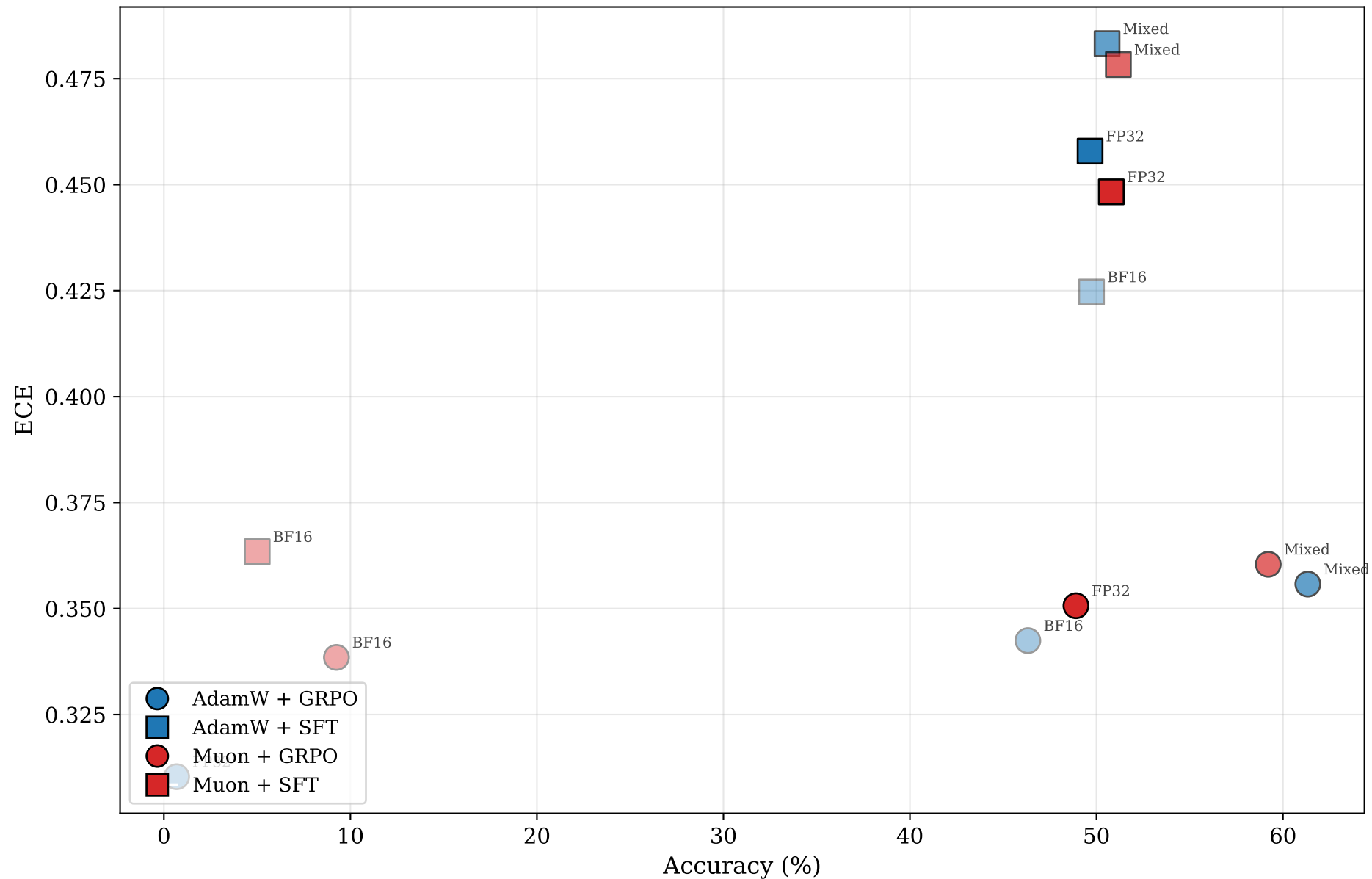
Accuracy vs Calibration Error (color = optimizer, shape = objective, label = precision)
