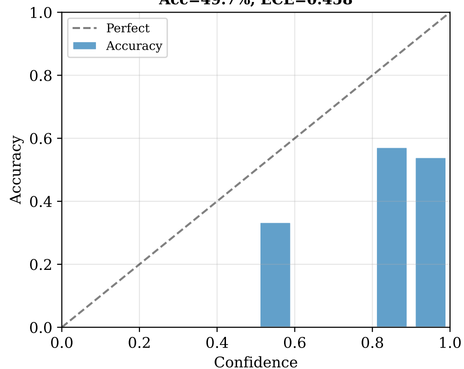
AdamW + SFT (FP32) Acc=49.7%, ECE=0.458
