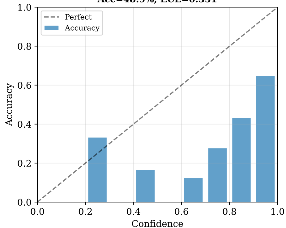
Muon + GRPO (FP32) Acc=48.9%, ECE=0.351
