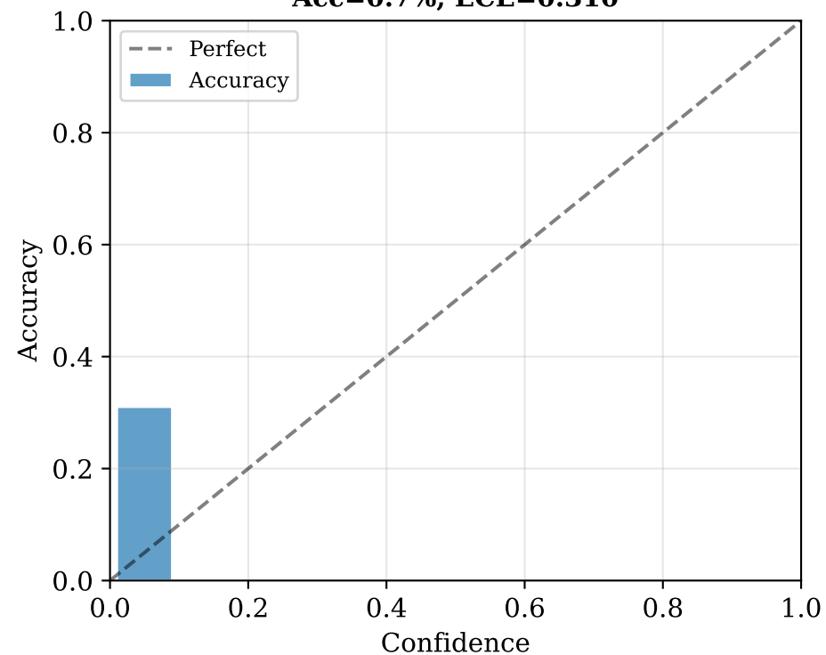
AdamW + GRPO (FP32) Acc=0.7%, ECE=0.310
