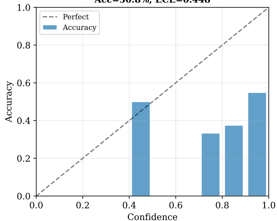
Muon + SFT (FP32) Acc=50.8%, ECE=0.448
