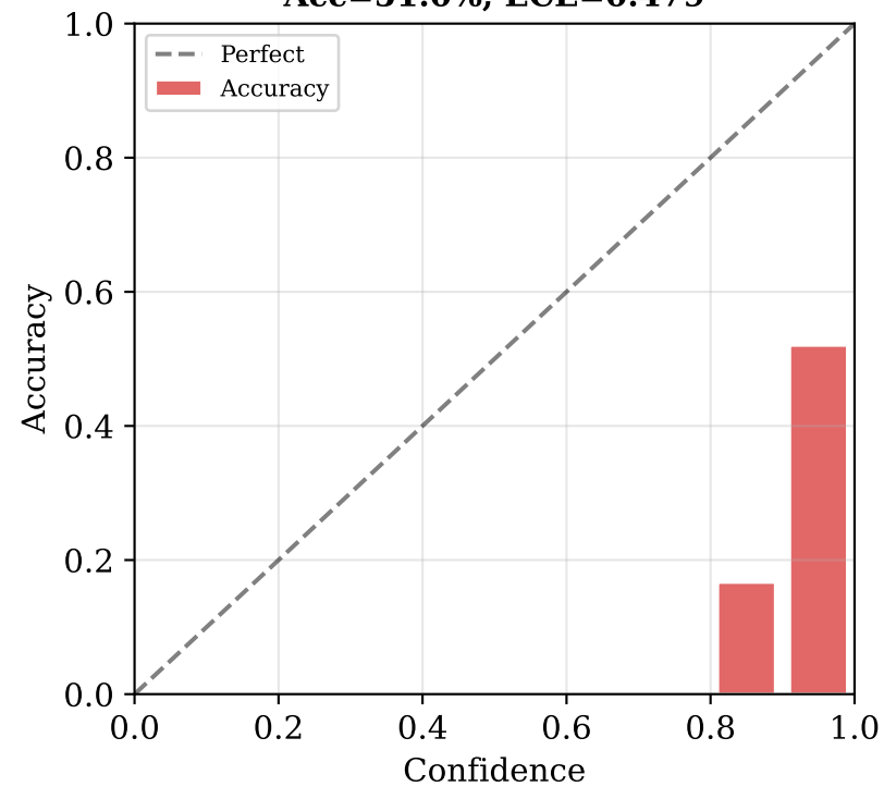
Muon + SFT Acc=51.0%, ECE=0.479
