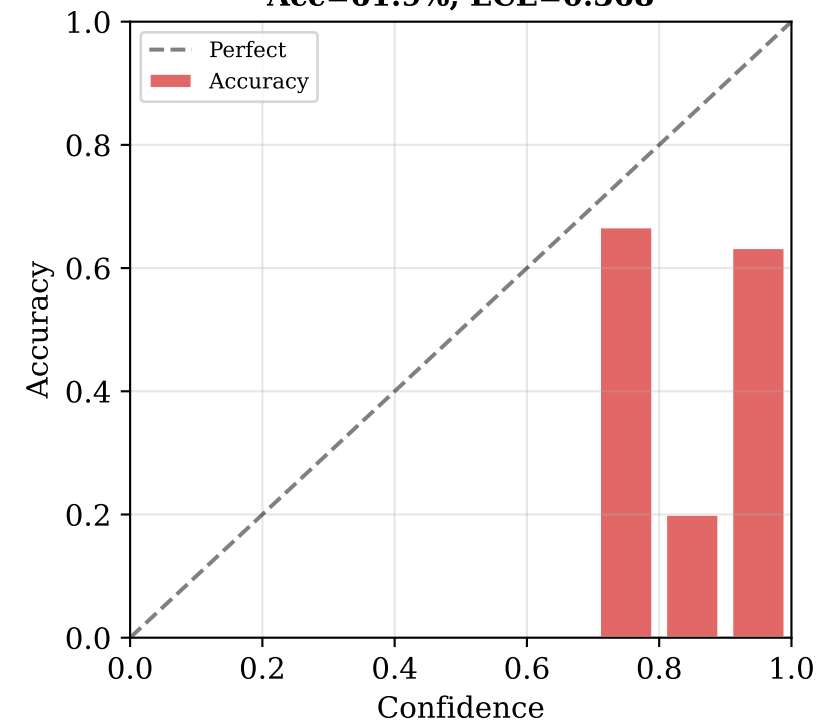
Muon + RS Acc=61.9%, ECE=0.368
