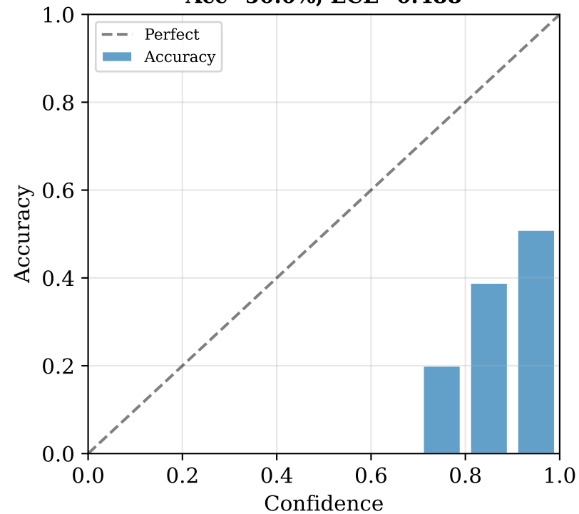
AdamW + SFT Acc=50.0%, ECE=0.488
