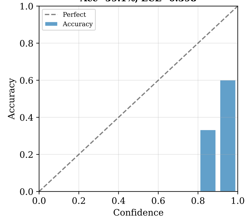
AdamW + RS Acc=59.1%, ECE=0.398
