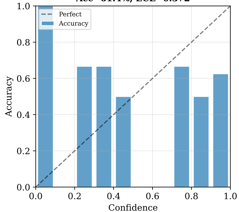
AdamW + GRPO Acc=61.4%, ECE=0.372
