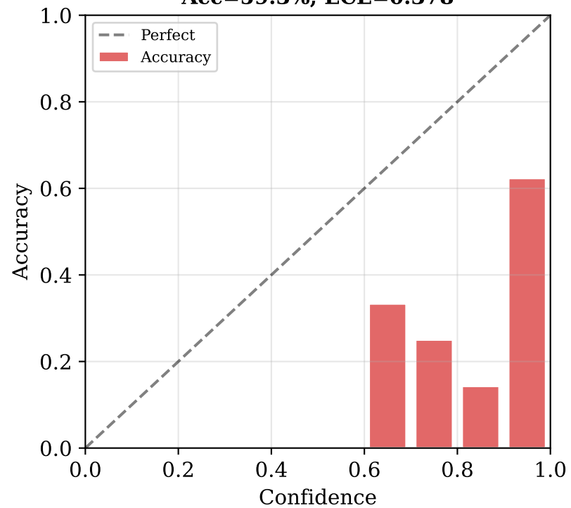
Muon + GRPO Acc=59.3%, ECE=0.378
