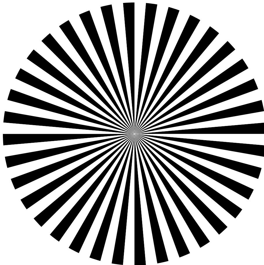
A5 MTF Siemens Star Target — Star Radius: 60 mm — Sectors: 72 — Fiducials at ( \pm 90 mm, \pm 59 mm)
