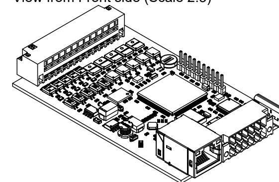
View from Front side (Scale 2:3)
