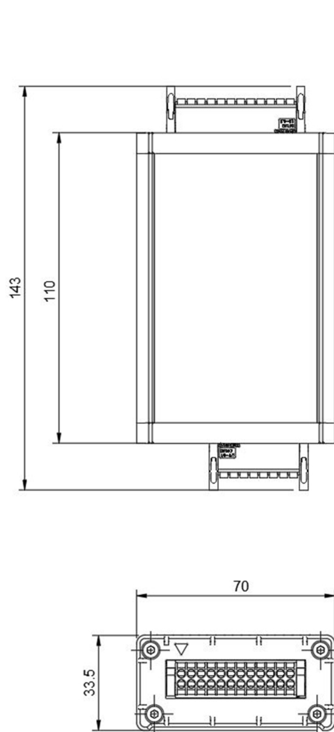
BareMetal PLC M
