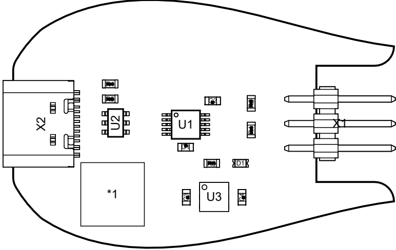
View from Top side (Scale 5:2)
