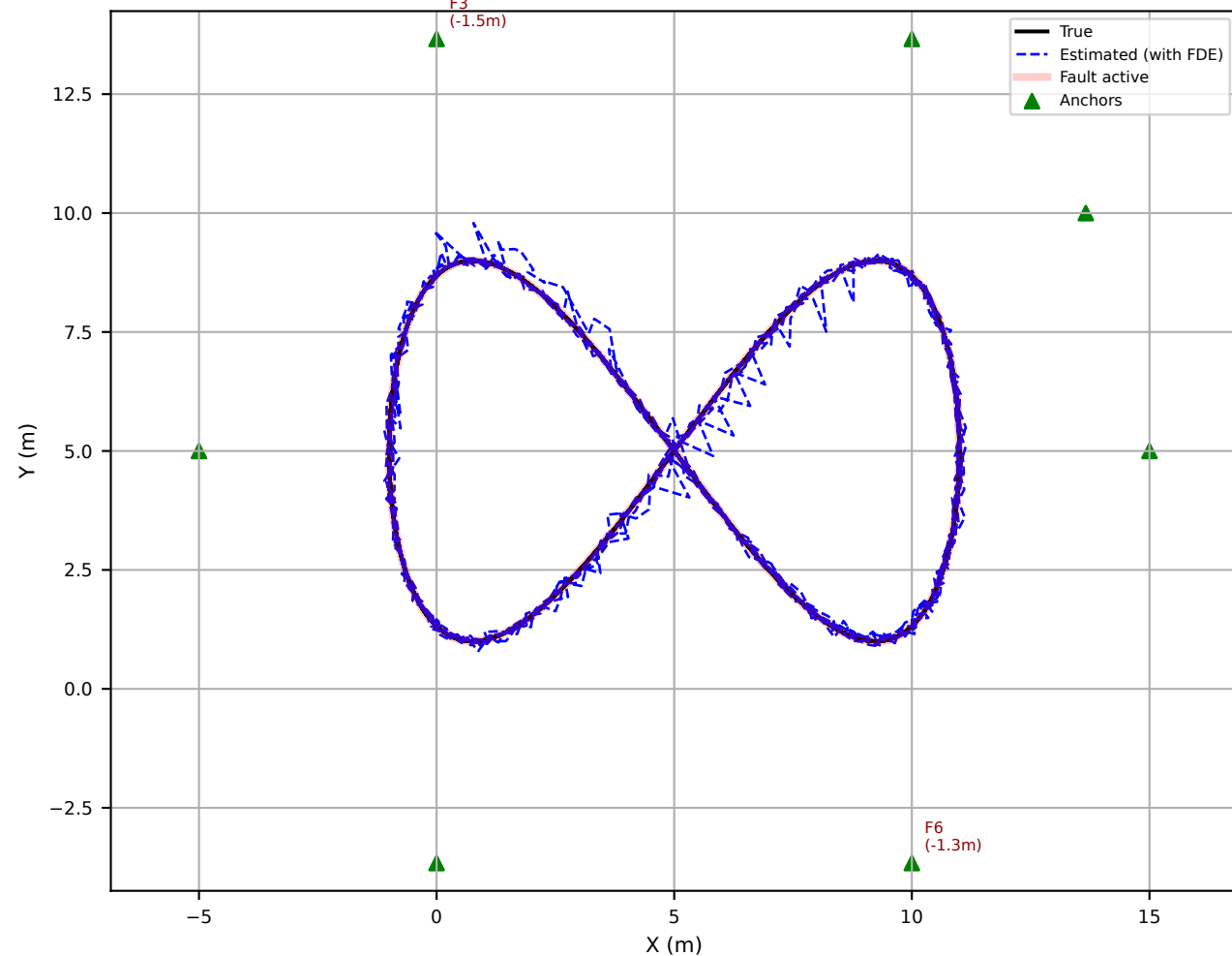
Trajectory with Time-Varying Faults and FDE
