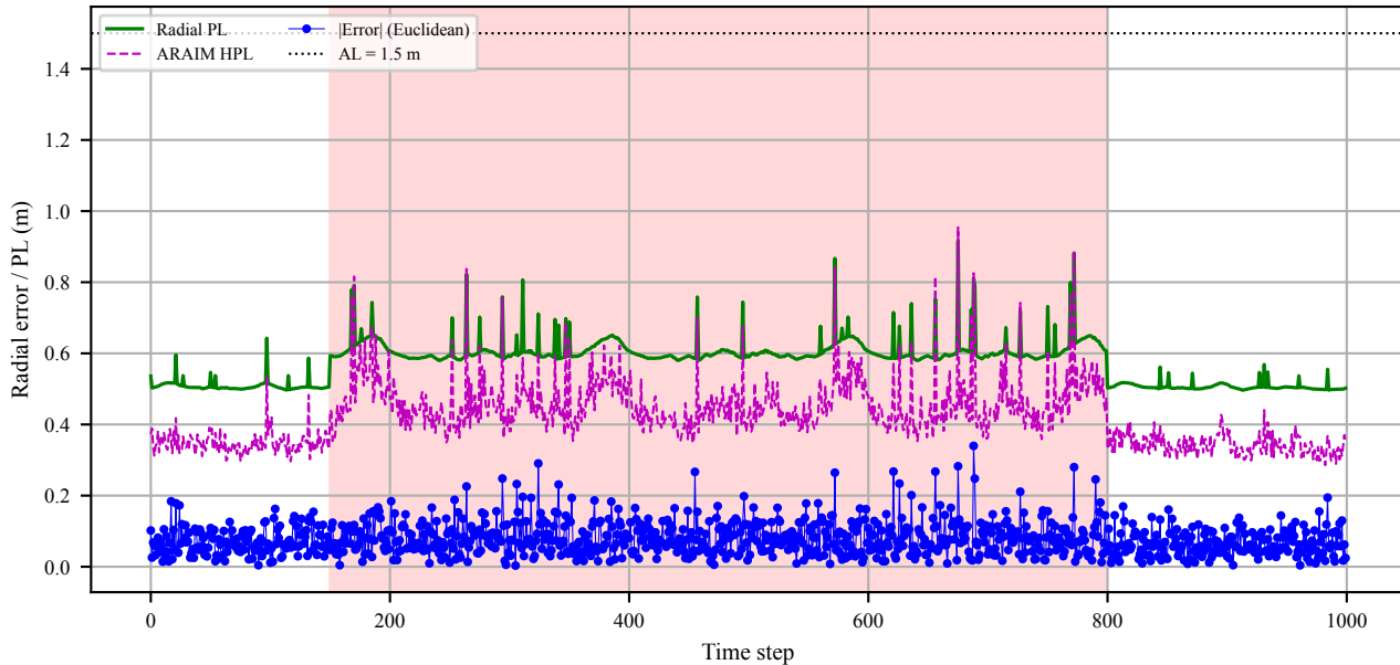
Radial Error vs. Protection Levels
