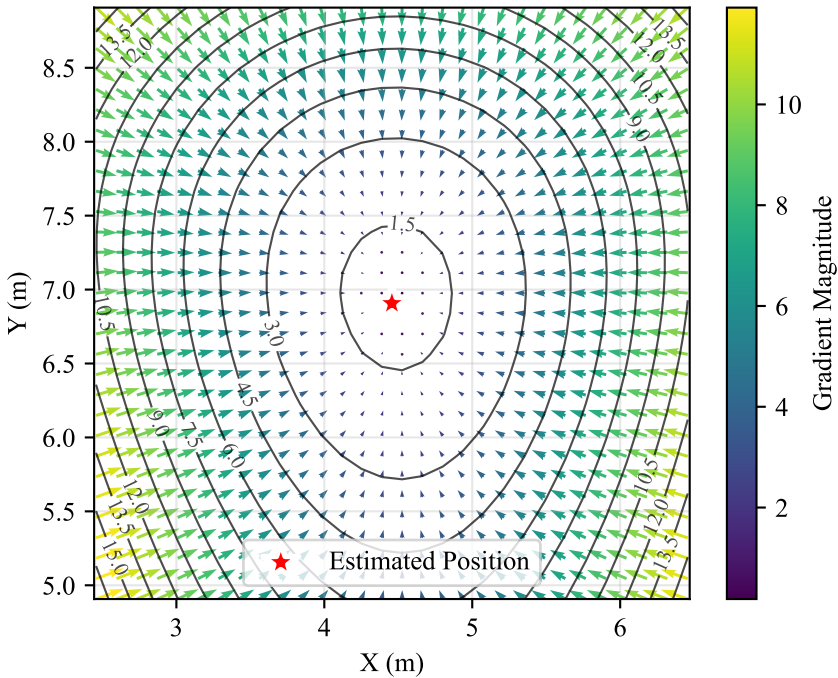
Gradient Field with Contours (Quiver + Contour lines)
