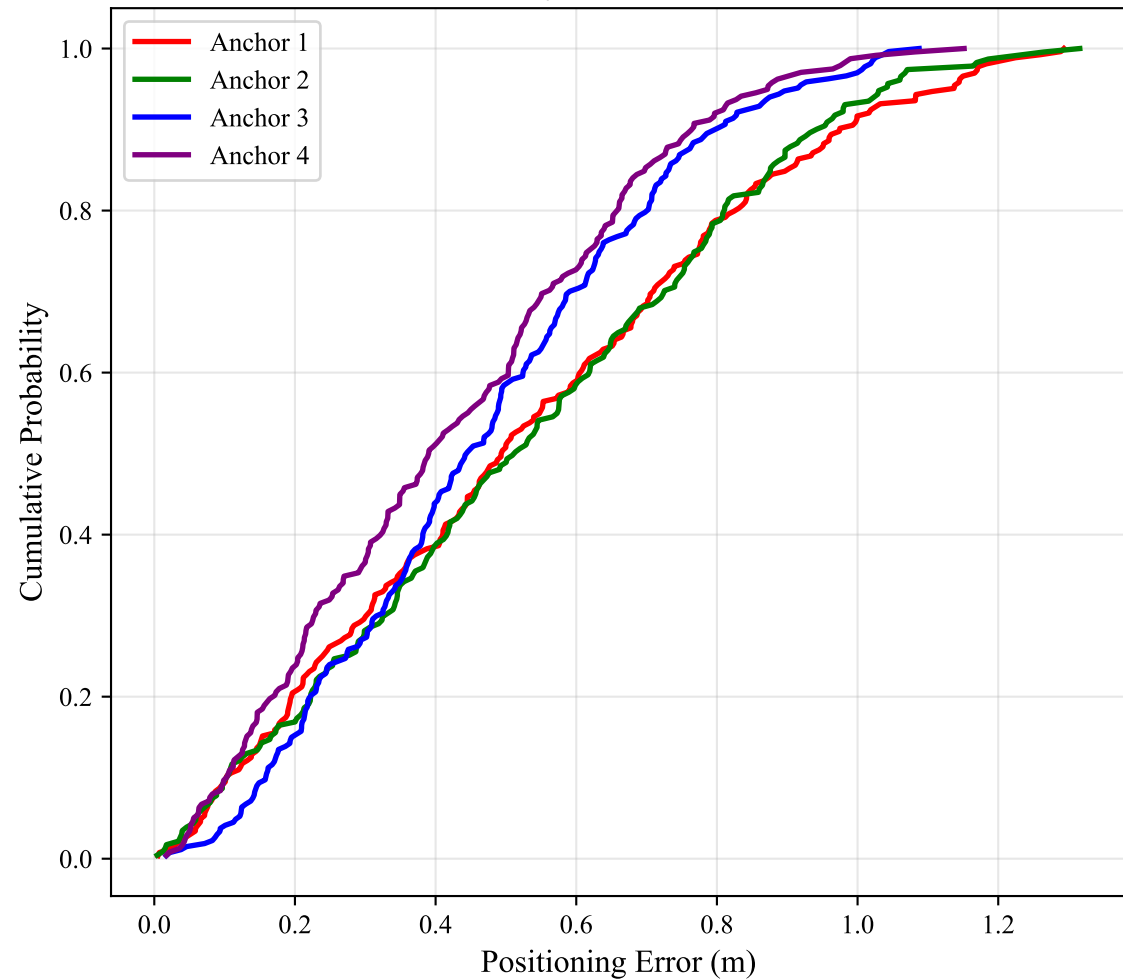
CDF by Biased Anchor
