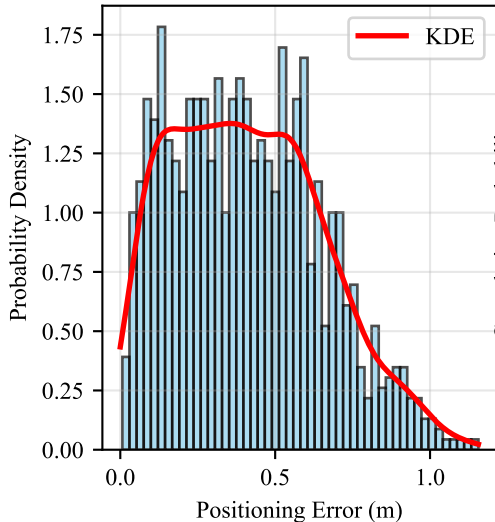
Probability Density Function (PDF) of Positioning Errors
