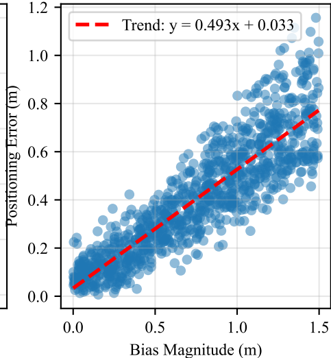
Positioning Error vs Bias Magnitude
