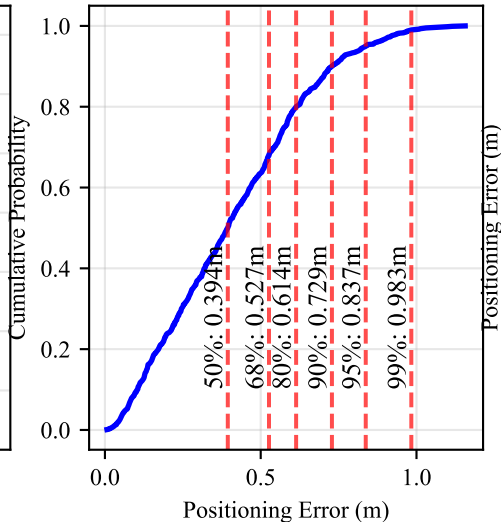
Cumulative Distribution Function (CDF) of Positioning Errors
