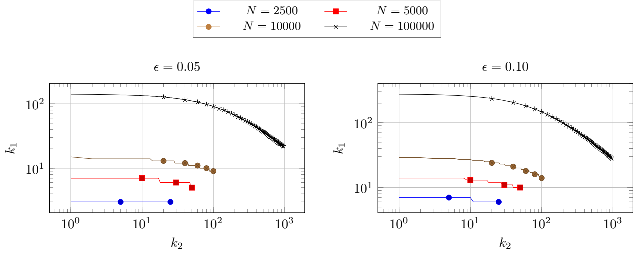
Figure 1: Side-by-side comparison of k_1 versus k_2 for k = 16 under different failure probabilities \epsilon .
