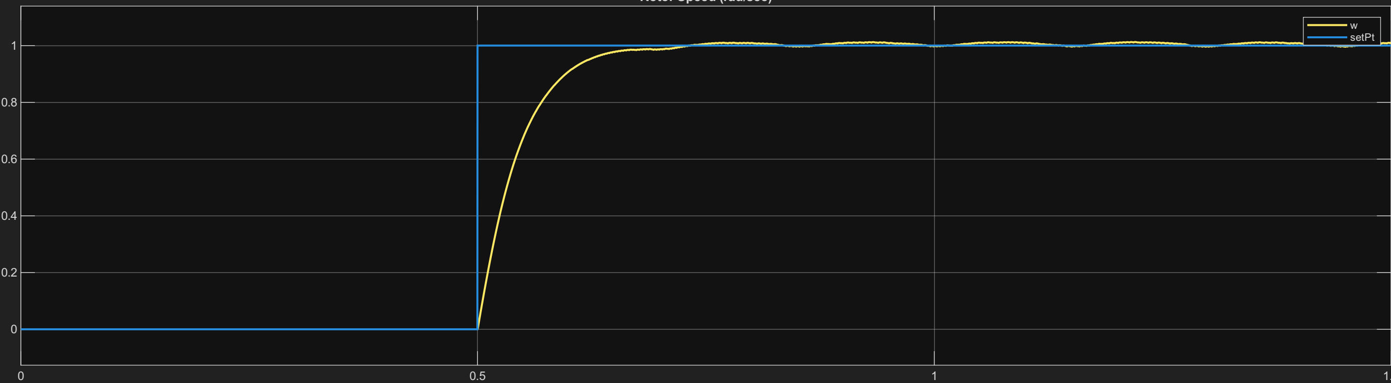
Rotor Speed (rad/sec)
