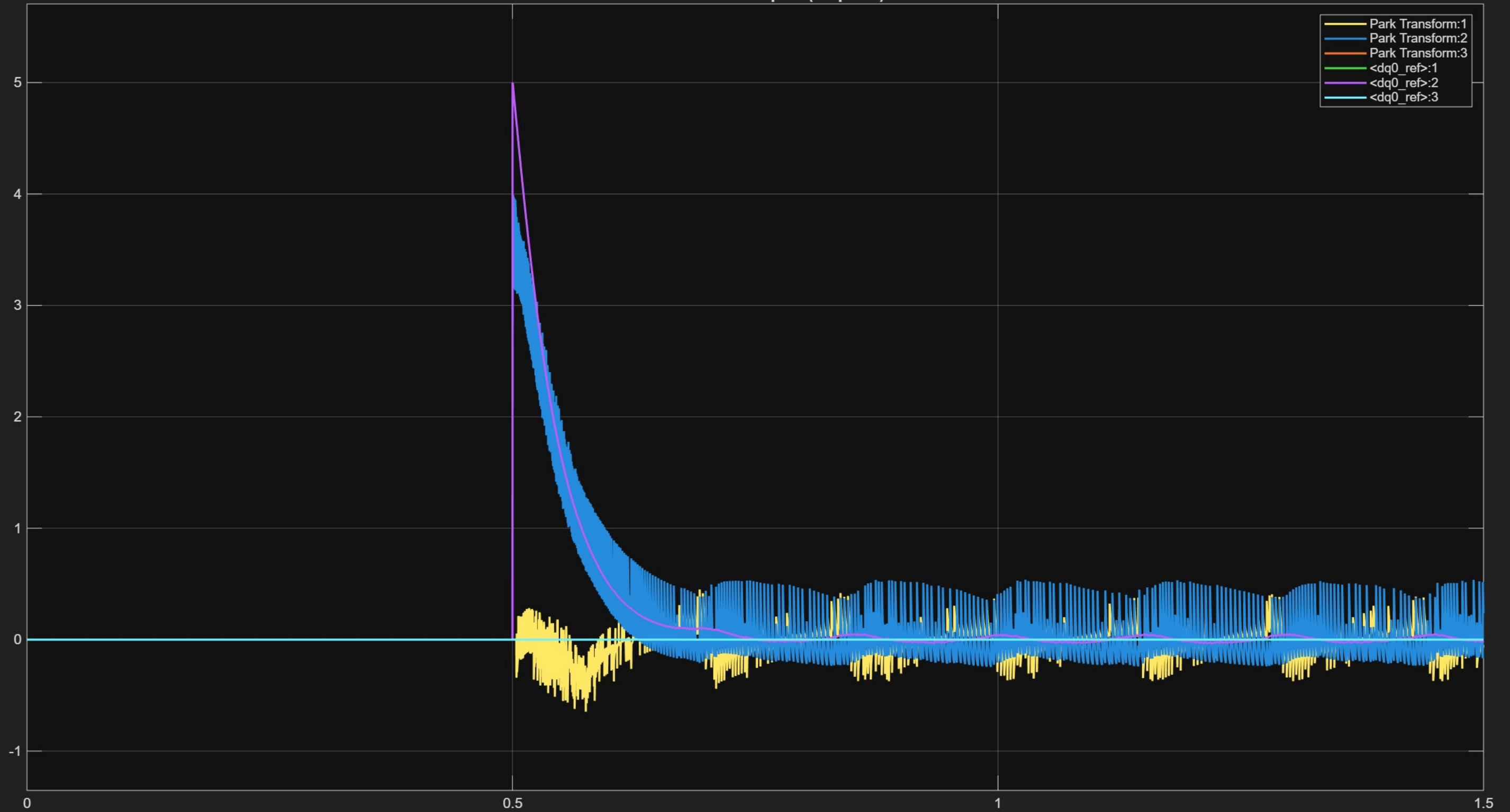
Park Transform Outputs (Amperes)
