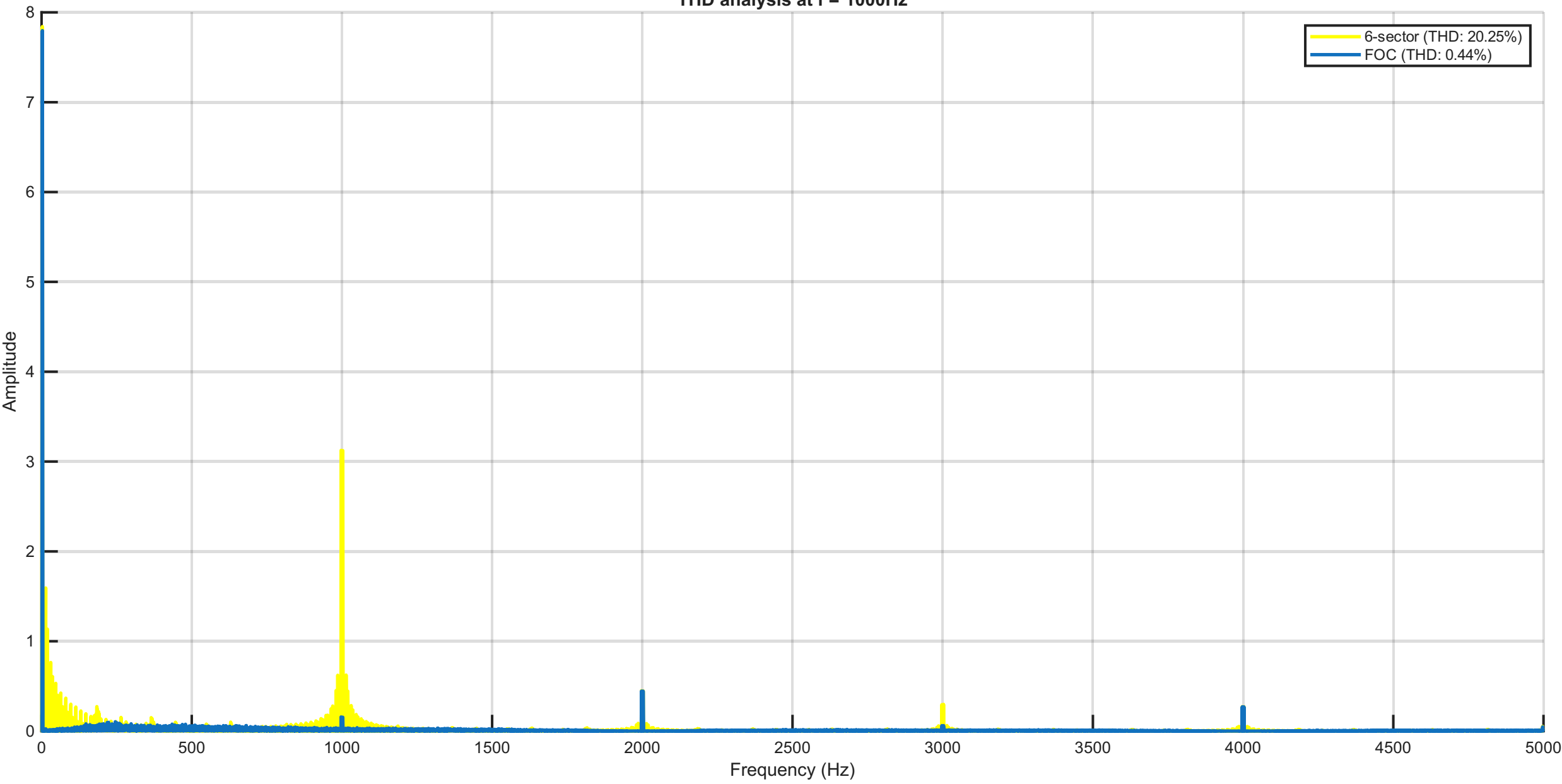
THD analysis at f = 1000Hz
