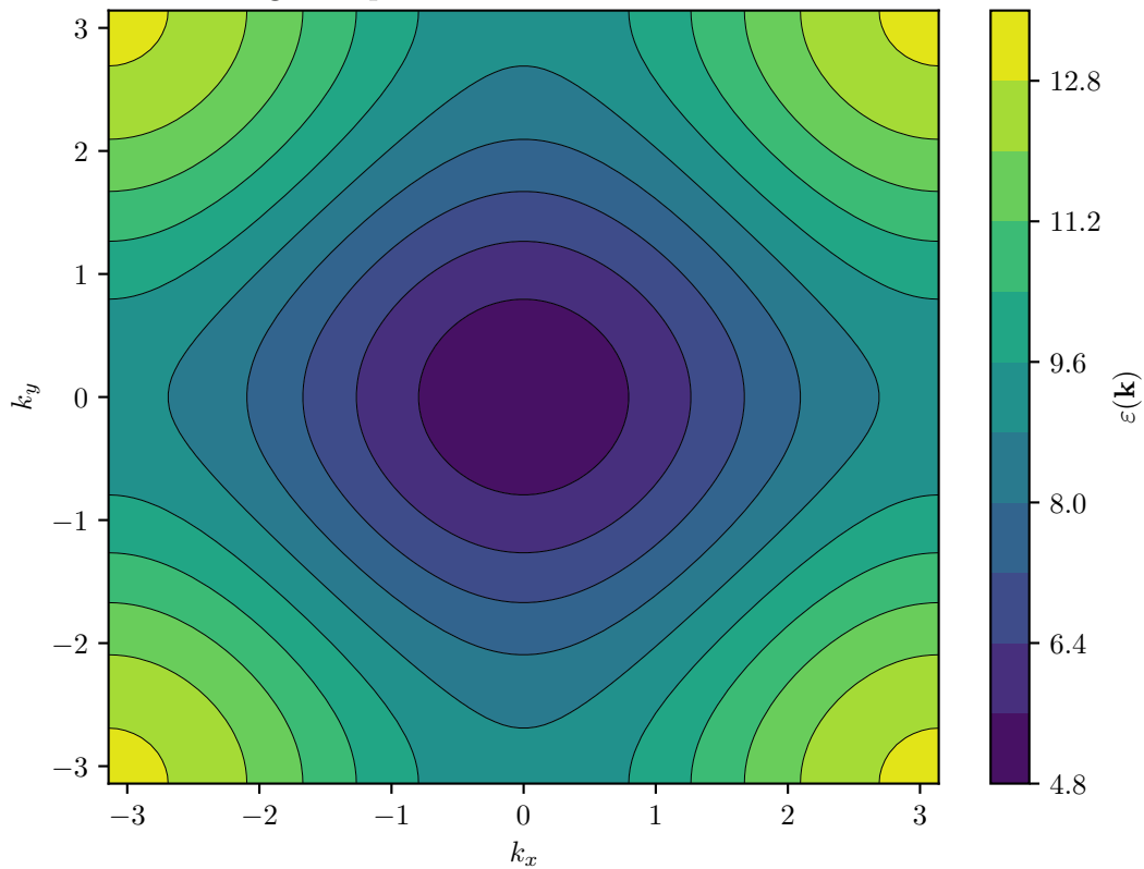
Magnon Spectrum of the 2D XXZ model
