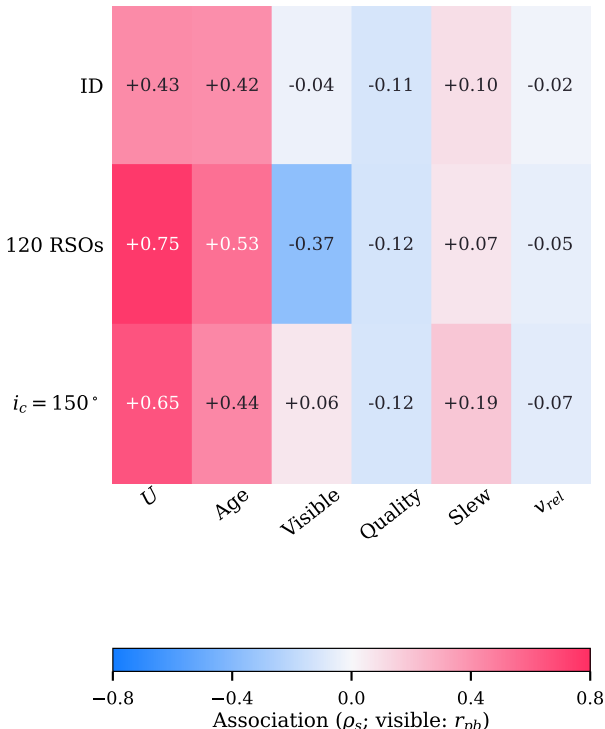
Mean attention-feature association
