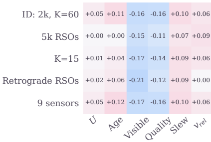
Head 1
