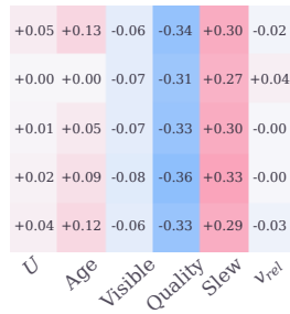
Head 4
