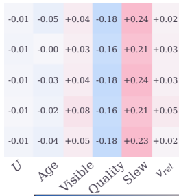
Head 2
