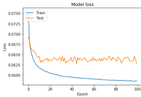
(a) MSE loss for 7DOF custom network with 3 layers and 100 hidden units each
