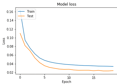
(a) Custom MSE loss for 7DOF custom network with 2 layers and 100 hidden units each
