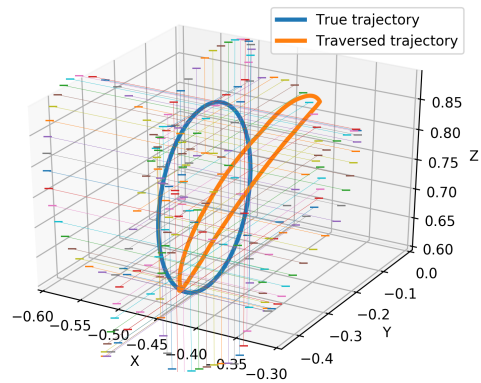
(b) Circular trajectory of end effector for best performing proposed network.
