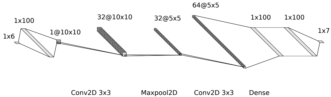
Figure 4: Proposed CNN architecture for 7DOF.
