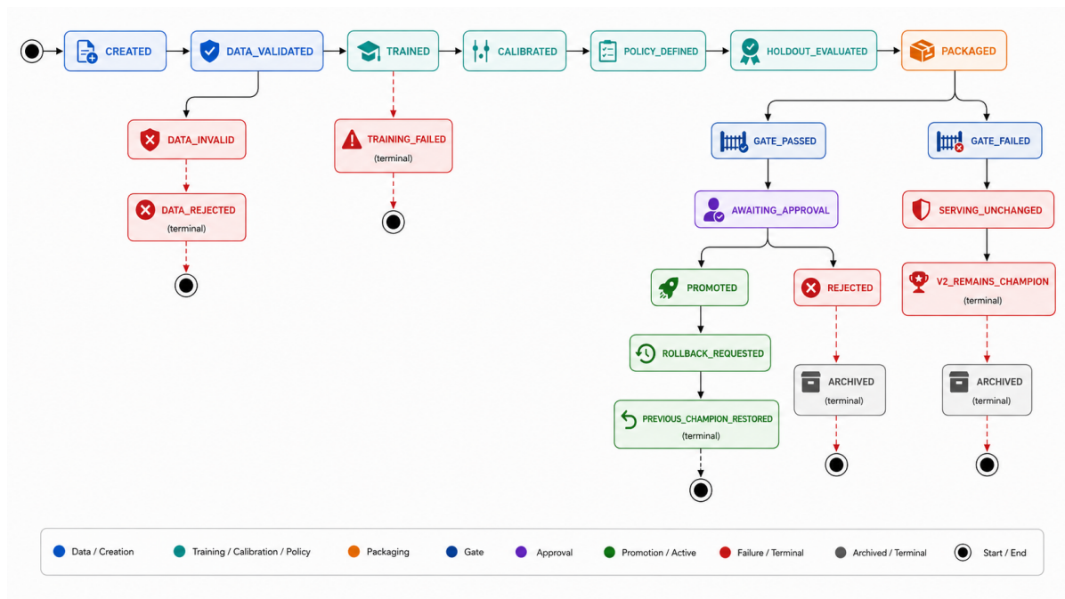
Figure 5.2: Promotion state machine. A failed candidate enters a failure/archive path while serving configuration remains unchanged.
