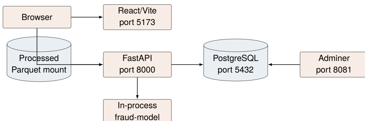
Figure B.1: Default application deployment. Adminer is optional; Spark training services are a separate Compose profile and are not needed for request-time scoring.
