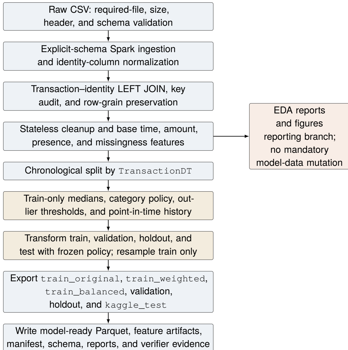
Figure 4.1: Detailed data processing pipeline (AS-BUILT). The canonical dataset names and output contract are shown explicitly; EDA is a reporting branch rather than a required transformation of model-ready data.
