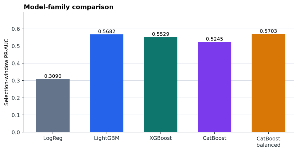
Figure 7.5: Model-family comparison (ARTIFACT-REPORTED). CatBoost balanced has the highest selection-window PR-AUC in the saved comparison artifact.
