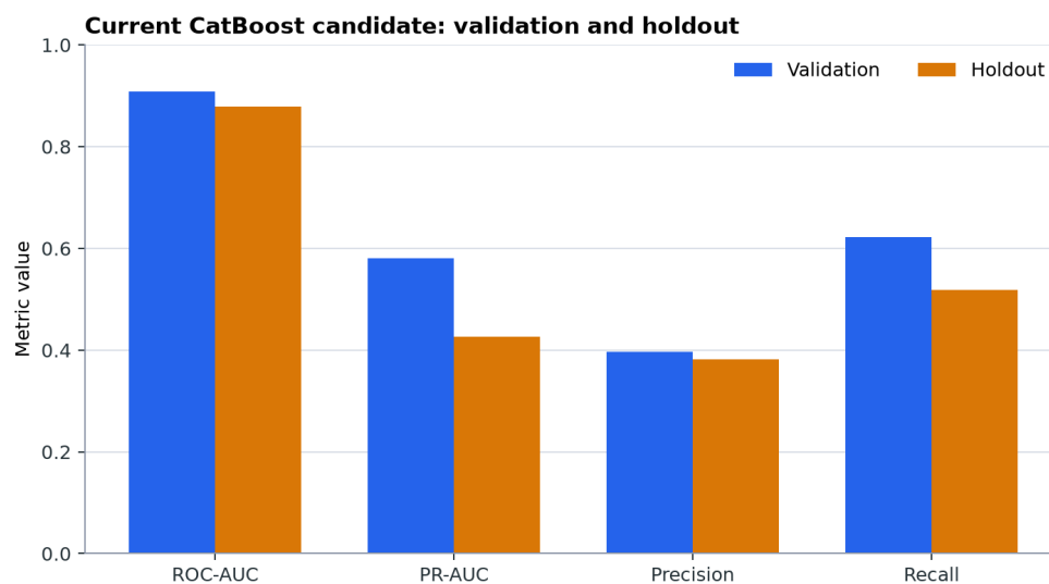
Figure 7.6: Current CatBoost candidate validation and holdout performance (ARTIFACT-REPORTED). Holdout ranking performance is lower than validation performance, with the largest decrease in PR-AUC.
