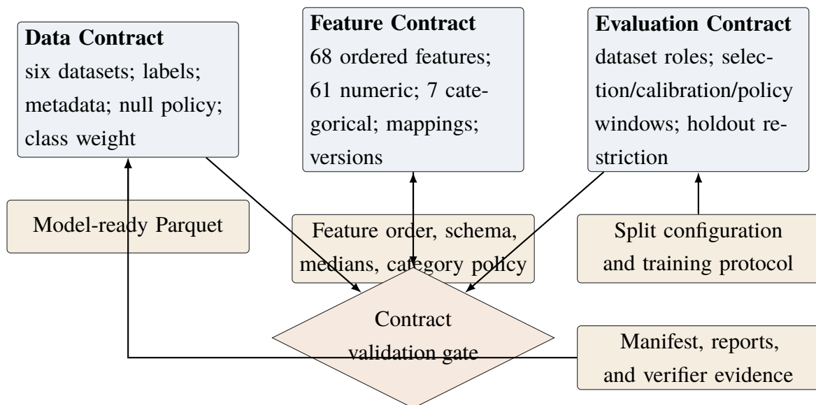
Figure 3.3: Data, feature, and evaluation contracts (HYBRID). Split configuration and the training protocol define the Evaluation Contract; manifests and verifiers provide validation evidence rather than defining policy.
