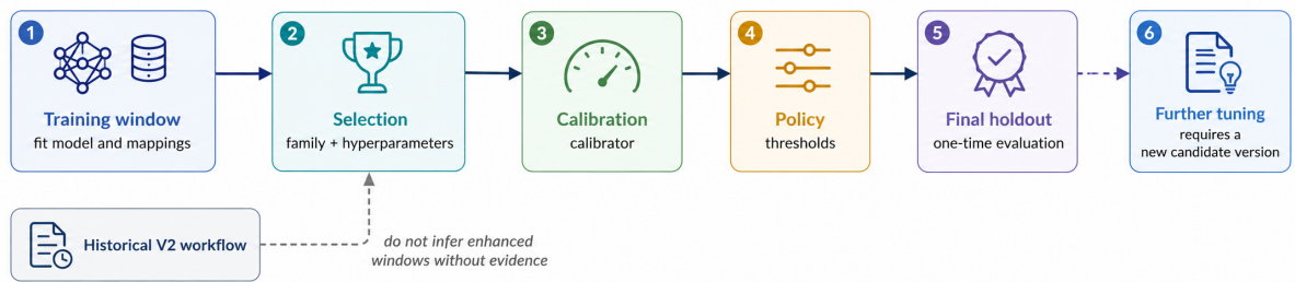
Figure 5.2: Temporal development windows (HYBRID). The enhanced candidate workflow separates selection, calibration, policy, and holdout roles; historical V2 evidence must not be rewritten as if it used every enhanced stage.
