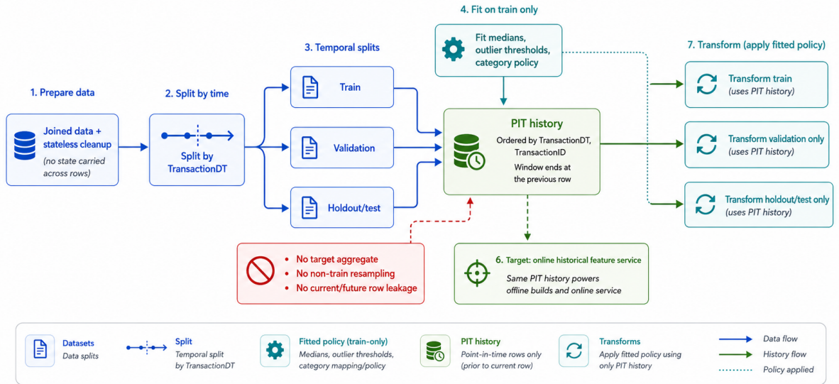
Figure 4.2: Leakage-controlled transformation flow (AS-BUILT). Learned preprocessing and historical lookups are fitted from the chronological training data and applied forward without current-row or future-row information.
