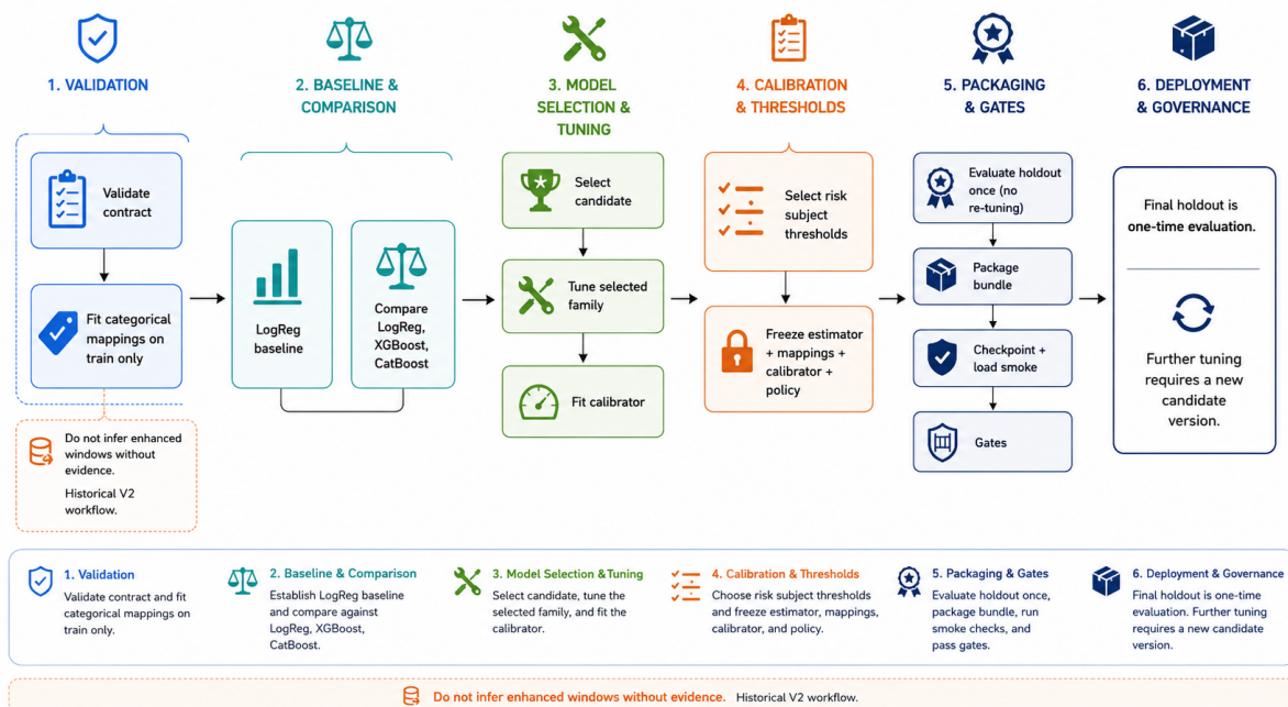
Figure 5.1: Model training lifecycle (HYBRID). The visual separates validation, comparison, selection/tuning, calibration/thresholds, packaging/gates, and governance. Spark provides distributed data preparation; estimator fitting is single-node Python training after the Parquet-to-Pandas boundary.
