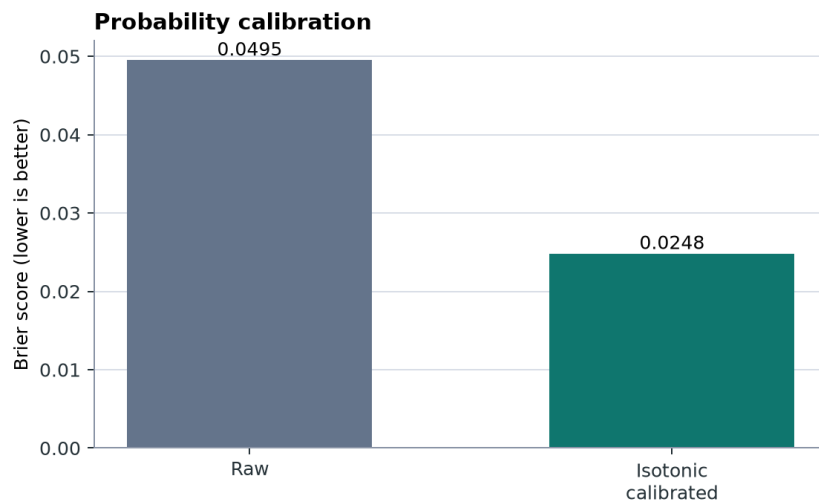
Figure 7.8: Raw versus isotonic-calibrated holdout Brier score (ARTIFACT-REPORTED). The lower calibrated score indicates improved probability calibration.
