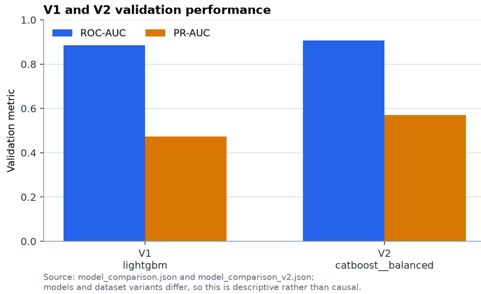
Figure B.2: Historical model artifact validation comparison.
