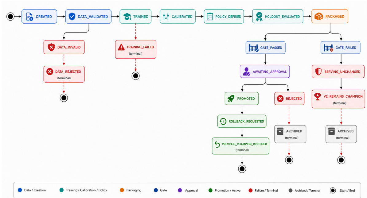
Figure 5.3: Promotion state machine (HYBRID). A failed candidate enters a failure/archive path; it does not transition into V2. Serving configuration remains unchanged until an approved update is made.
