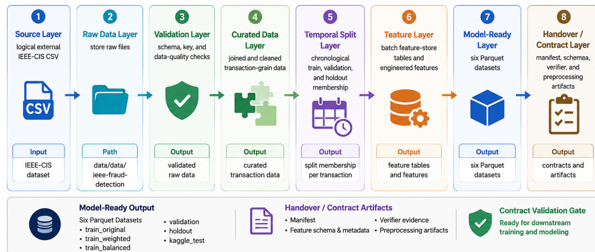
Figure 3.2: Layered data architecture (AS-BUILT). Curated data and temporal split membership are separate layers; preprocessing artifacts belong to the handover/contract layer rather than the feature layer.
