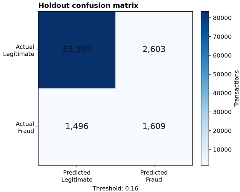
Figure 7.7: Holdout confusion matrix at the review threshold of 0.16 (ARTIFACT-REPORTED). The candidate detects 1,609 fraud cases and misses 1,496, while 2,603 legitimate transactions are flagged as positive.
