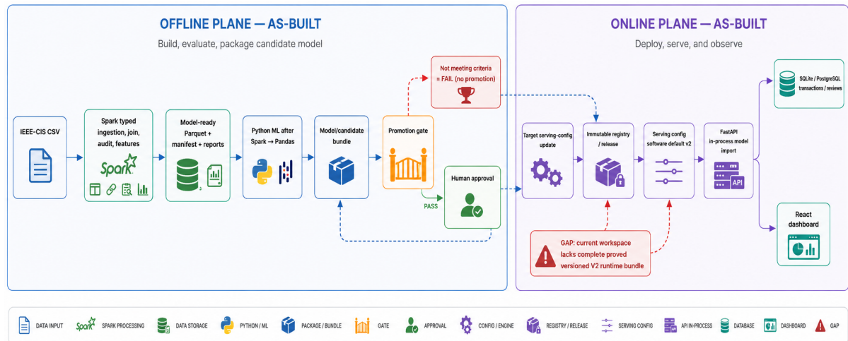
Figure 3.1: Overall system architecture (HYBRID). Solid lines are implemented and evidenced; dashed lines are proposed or partially enforced. The failed-candidate path leaves serving unchanged and retains the configured champion.
